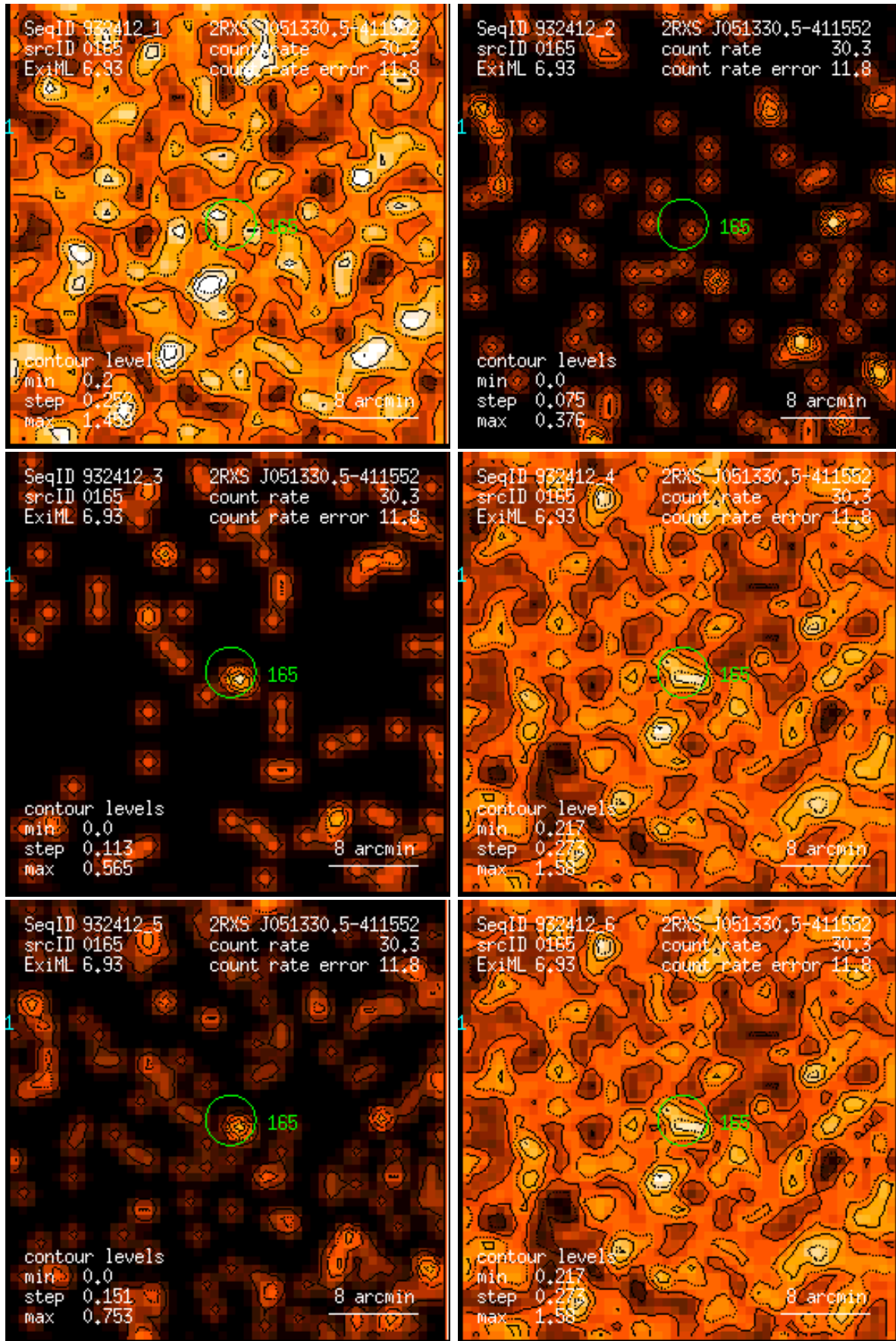
Figure 165: RASS 932412: detection 0165: band rate images, Gaussian filter: (1) PSPC channels 11 – 41, (2) 52 – 90, (3) 91 – 201, (4) 11 – 235, (5) 52 – 201, (6) 11 – 201. Broad band rates in counts/ks. Band rate contour levels in counts/ks/arcmin 2 .
