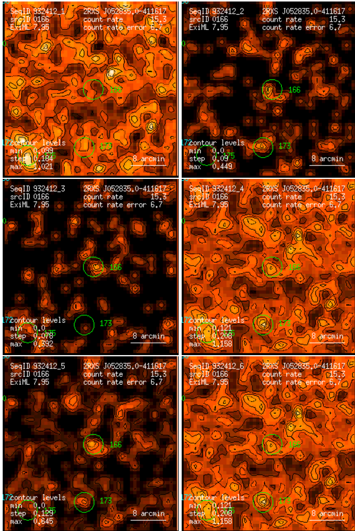
Figure 166: RASS 932412: detection 0166: band rate images, Gaussian filter: (1) PSPC channels 11 – 41, (2) 52 – 90, (3) 91 – 201, (4) 11 – 235, (5) 52 – 201, (6) 11 – 201. Broad band rates in counts/ks. Band rate contour levels in counts/ks/arcmin 2 .
