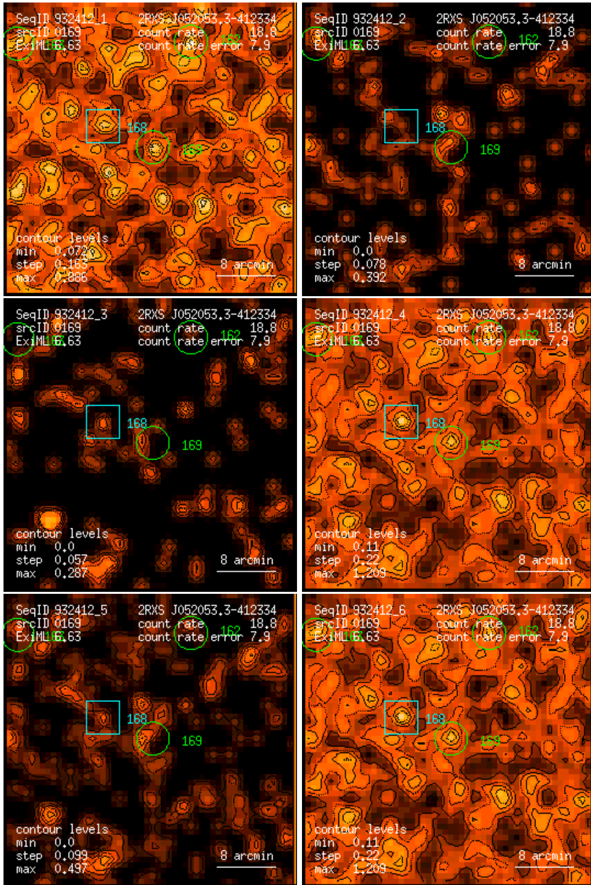
Figure 169: RASS 932412: detection 0169: band rate images, Gaussian filter: (1) PSPC channels 11 – 41, (2) 52 – 90, (3) 91 – 201, (4) 11 – 235, (5) 52 – 201, (6) 11 – 201. Broad band rates in counts/ks. Band rate contour levels in counts/ks/arcmin 2 .
