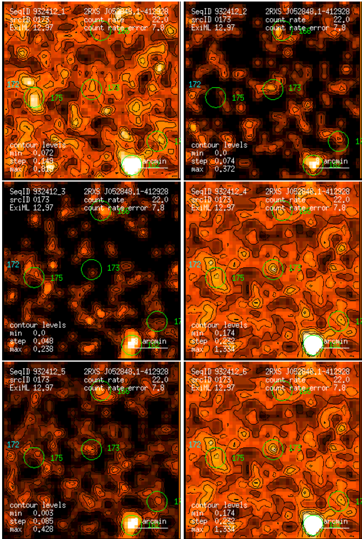
Figure 173: RASS 932412: detection 0173: band rate images, Gaussian filter: (1) PSPC channels 11 – 41, (2) 52 – 90, (3) 91 – 201, (4) 11 – 235, (5) 52 – 201, (6) 11 – 201. Broad band rates in counts/ks. Band rate contour levels in counts/ks/arcmin 2 .
