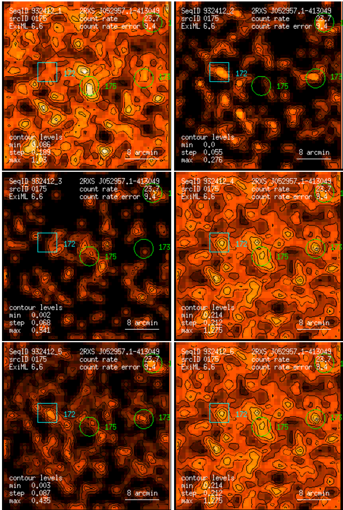
Figure 175: RASS 932412: detection 0175: band rate images, Gaussian filter: (1) PSPC channels 11 – 41, (2) 52 – 90, (3) 91 – 201, (4) 11 – 235, (5) 52 – 201, (6) 11 – 201. Broad band rates in counts/ks. Band rate contour levels in counts/ks/arcmin 2 .
