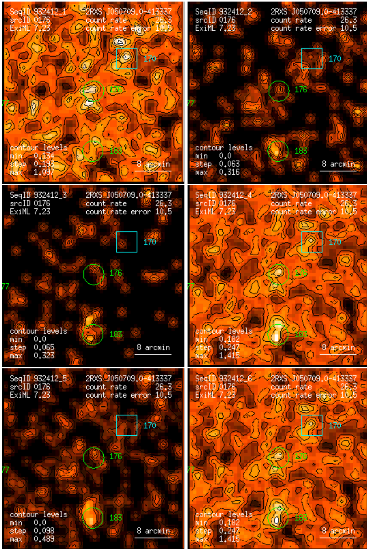
Figure 176: RASS 932412: detection 0176: band rate images, Gaussian filter: (1) PSPC channels 11 – 41, (2) 52 – 90, (3) 91 – 201, (4) 11 – 235, (5) 52 – 201, (6) 11 – 201. Broad band rates in counts/ks. Band rate contour levels in counts/ks/arcmin 2 .
