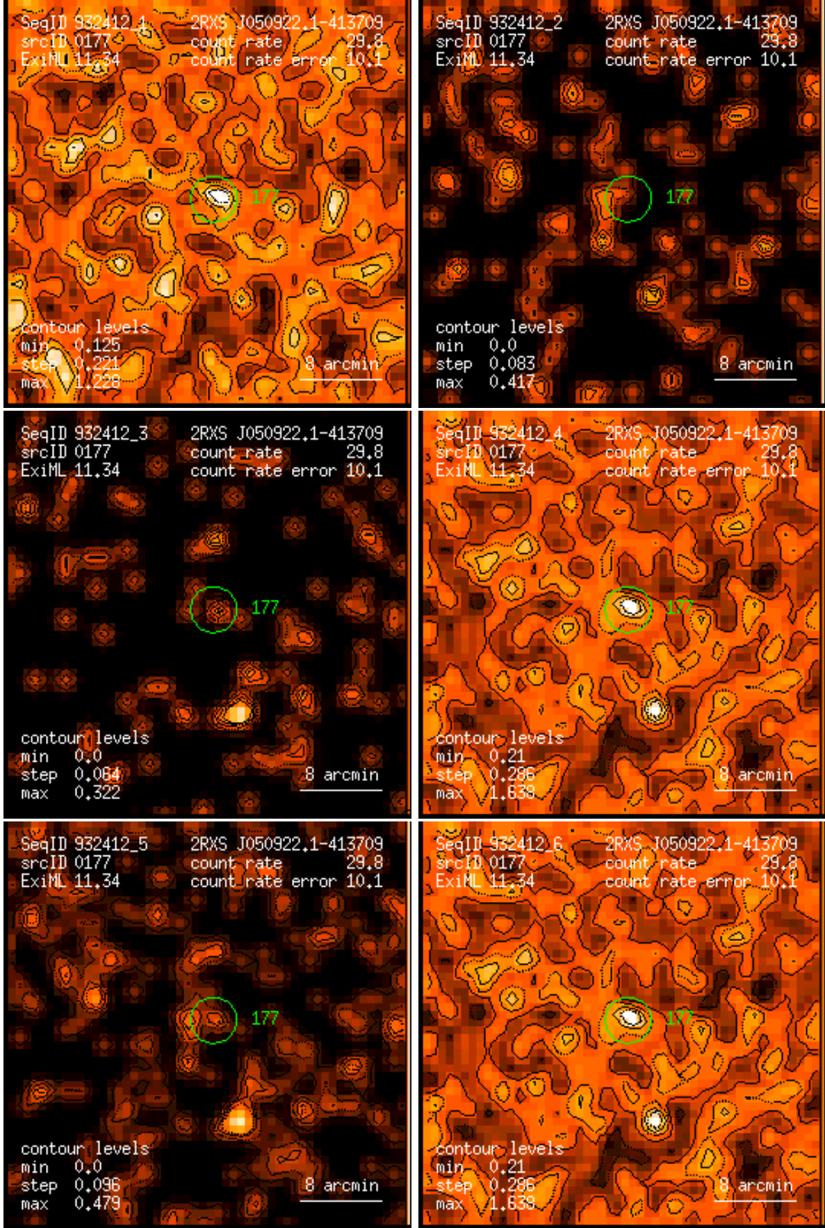
Figure 177: RASS 932412: detection 0177: band rate images, Gaussian filter: (1) PSPC channels 11 – 41, (2) 52 – 90, (3) 91 – 201, (4) 11 – 235, (5) 52 – 201, (6) 11 – 201. Broad band rates in counts/ks. Band rate contour levels in counts/ks/arcmin 2 .
