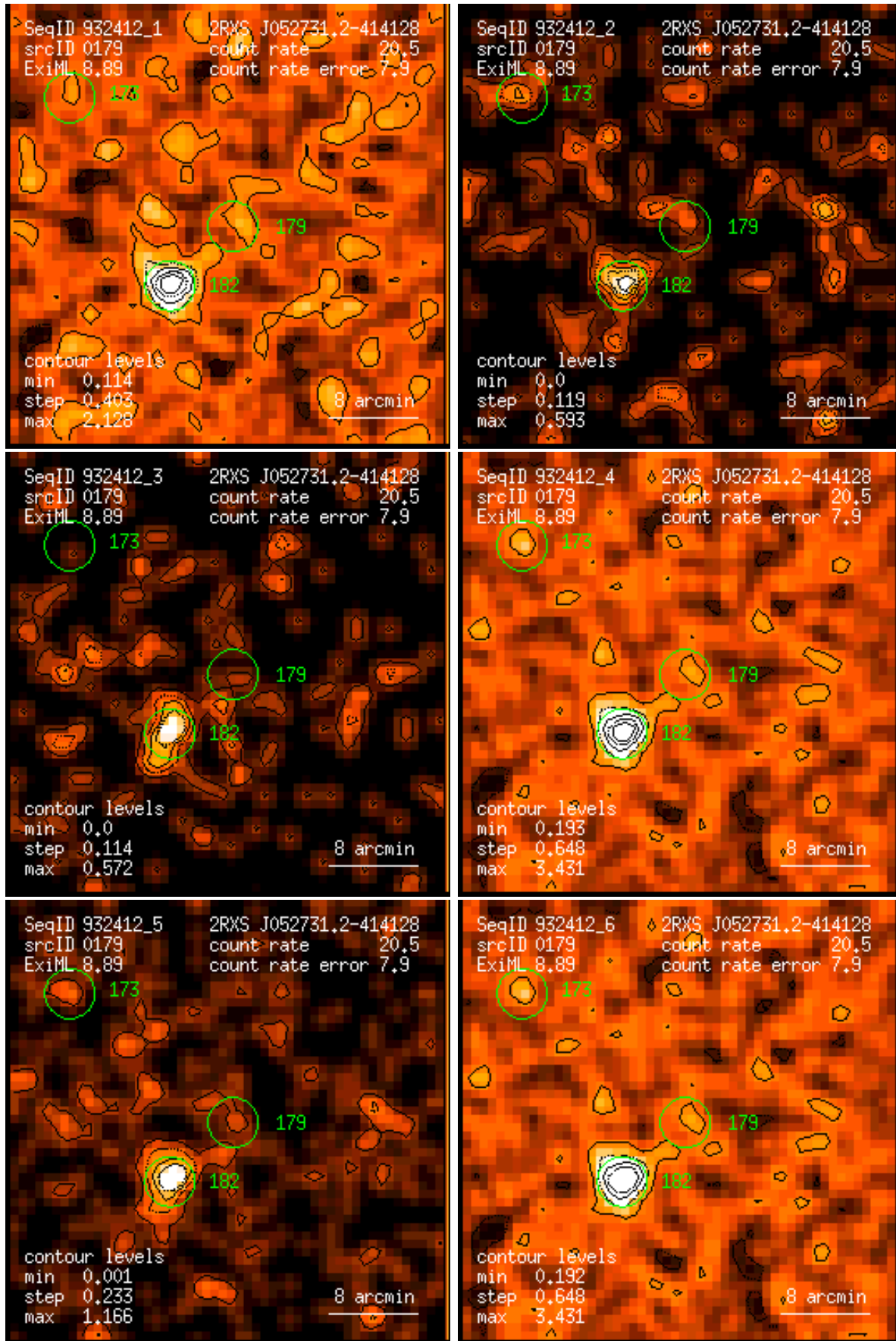
Figure 179: RASS 932412: detection 0179: band rate images, Gaussian filter: (1) PSPC channels 11 – 41, (2) 52 – 90, (3) 91 – 201, (4) 11 – 235, (5) 52 – 201, (6) 11 – 201. Broad band rates in counts/ks. Band rate contour levels in counts/ks/arcmin 2 .
