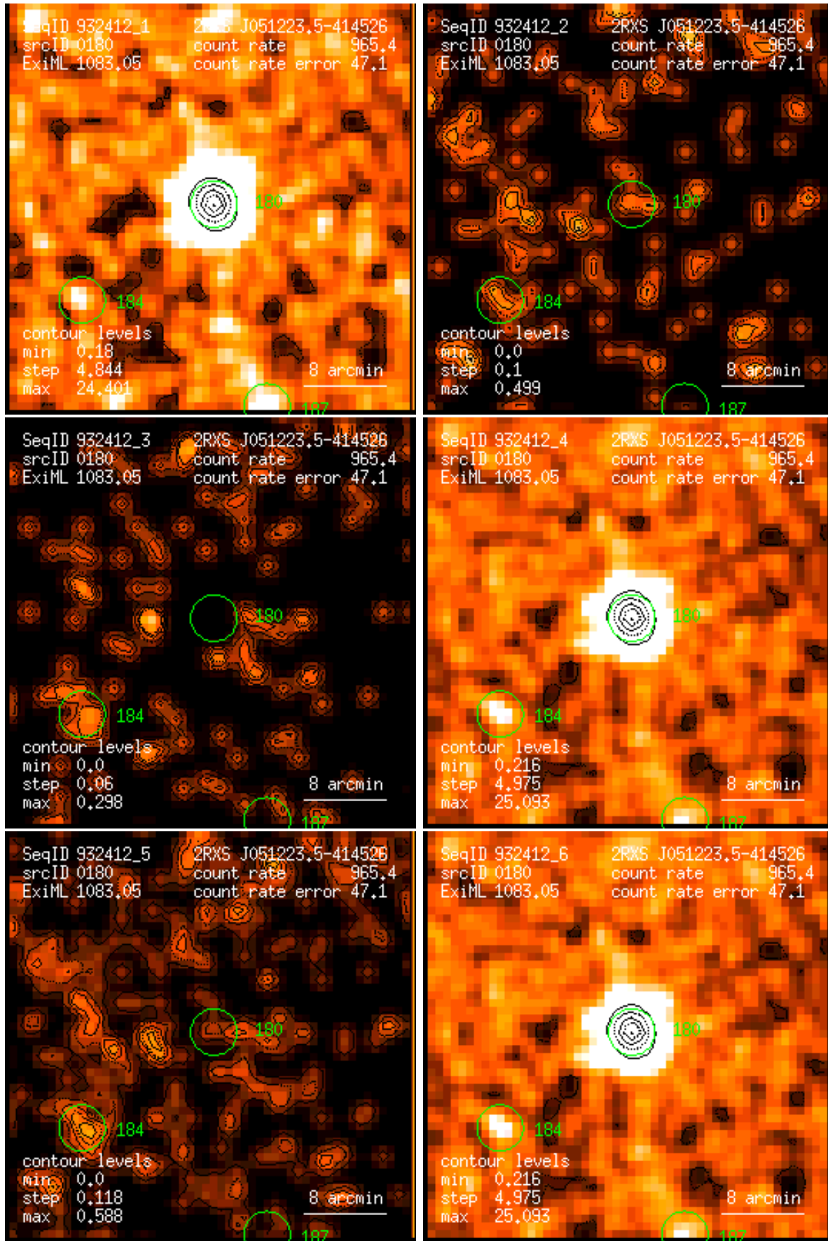
Figure 180: RASS 932412: detection 0180: band rate images, Gaussian filter: (1) PSPC channels 11 – 41, (2) 52 – 90, (3) 91 – 201, (4) 11 – 235, (5) 52 – 201, (6) 11 – 201. Broad band rates in counts/ks. Band rate contour levels in counts/ks/arcmin 2 .
