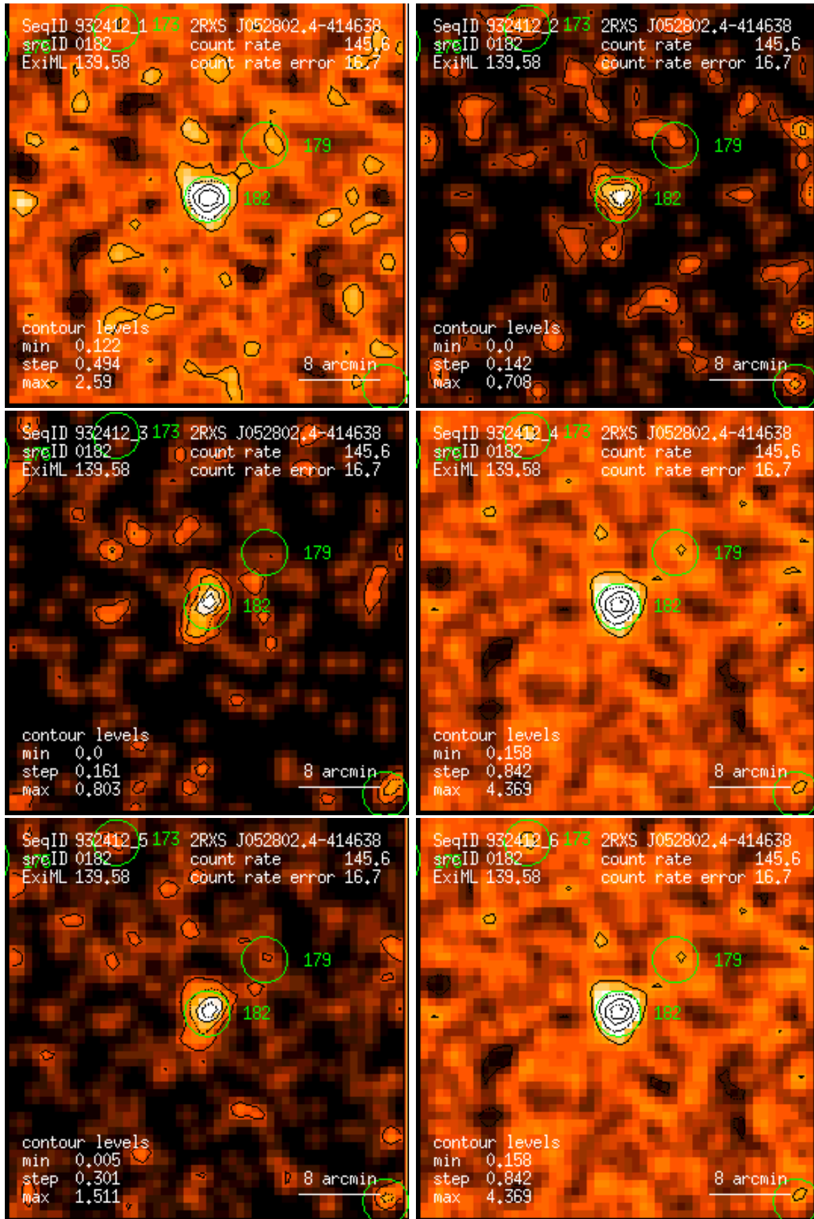
Figure 182: RASS 932412: detection 0182: band rate images, Gaussian filter: (1) PSPC channels 11 – 41, (2) 52 – 90, (3) 91 – 201, (4) 11 – 235, (5) 52 – 201, (6) 11 – 201. Broad band rates in counts/ks. Band rate contour levels in counts/ks/arcmin 2 .
