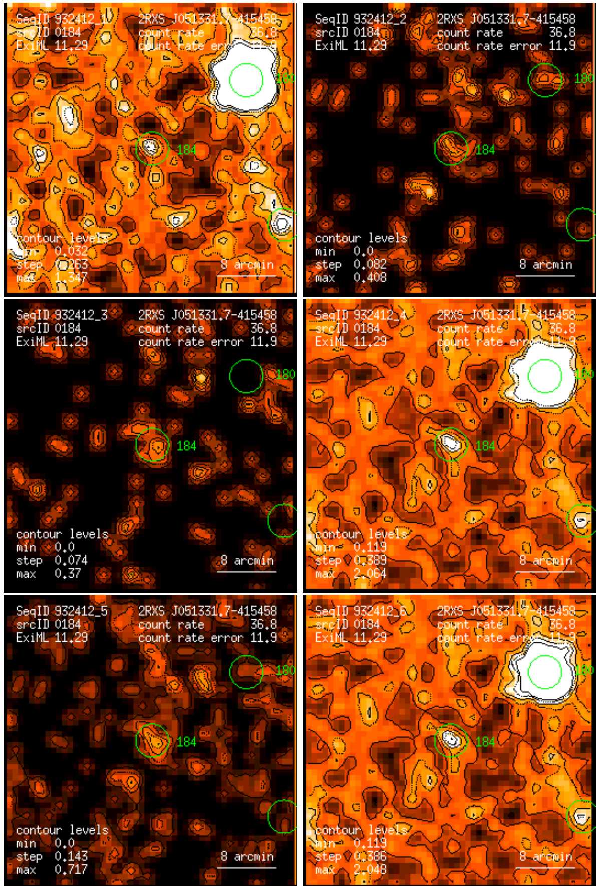
Figure 184: RASS 932412: detection 0184: band rate images, Gaussian filter: (1) PSPC channels 11 – 41, (2) 52 – 90, (3) 91 – 201, (4) 11 – 235, (5) 52 – 201, (6) 11 – 201. Broad band rates in counts/ks. Band rate contour levels in counts/ks/arcmin 2 .
