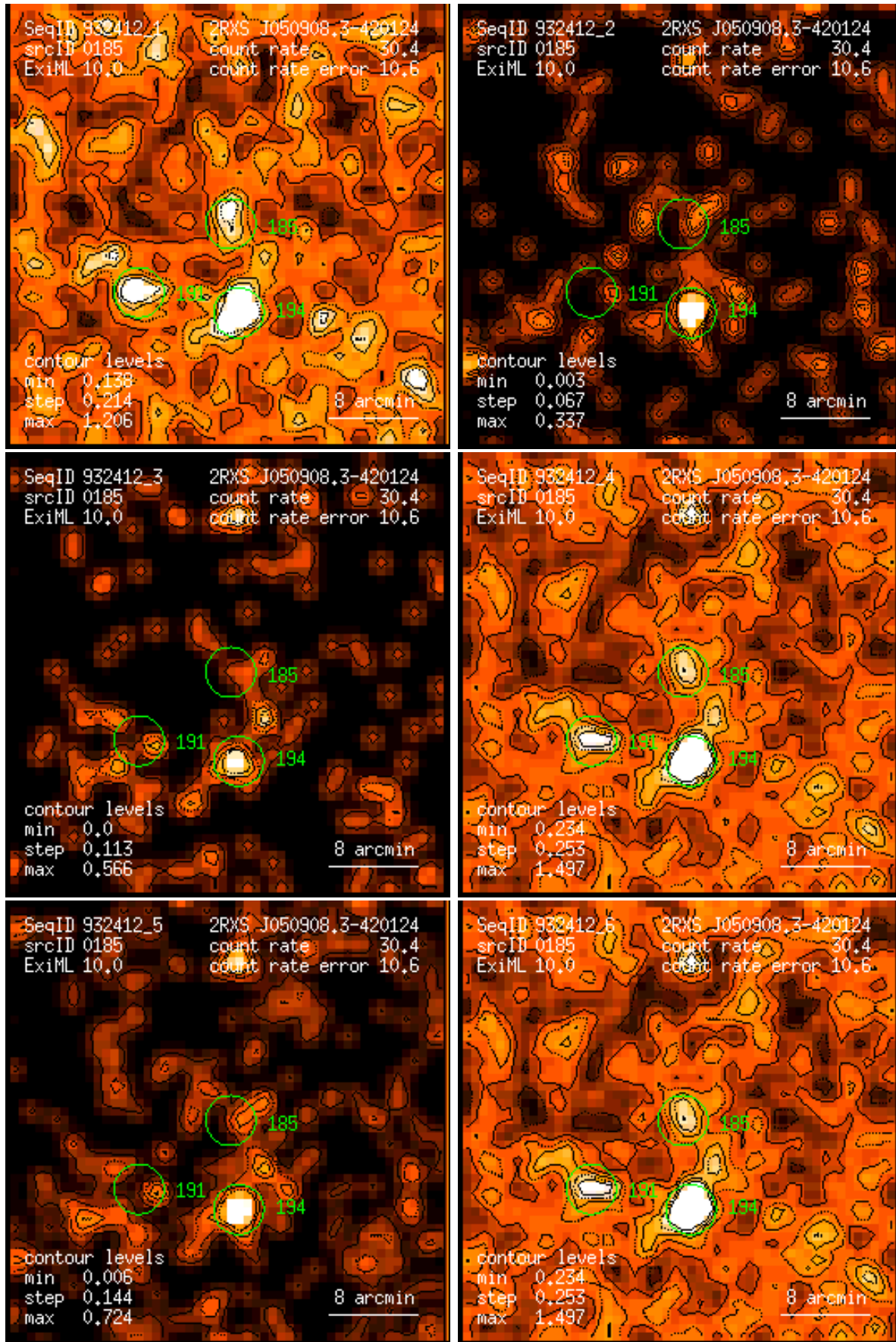
Figure 185: RASS 932412: detection 0185: band rate images, Gaussian filter: (1) PSPC channels 11 – 41, (2) 52 – 90, (3) 91 – 201, (4) 11 – 235, (5) 52 – 201, (6) 11 – 201. Broad band rates in counts/ks. Band rate contour levels in counts/ks/arcmin 2 .
