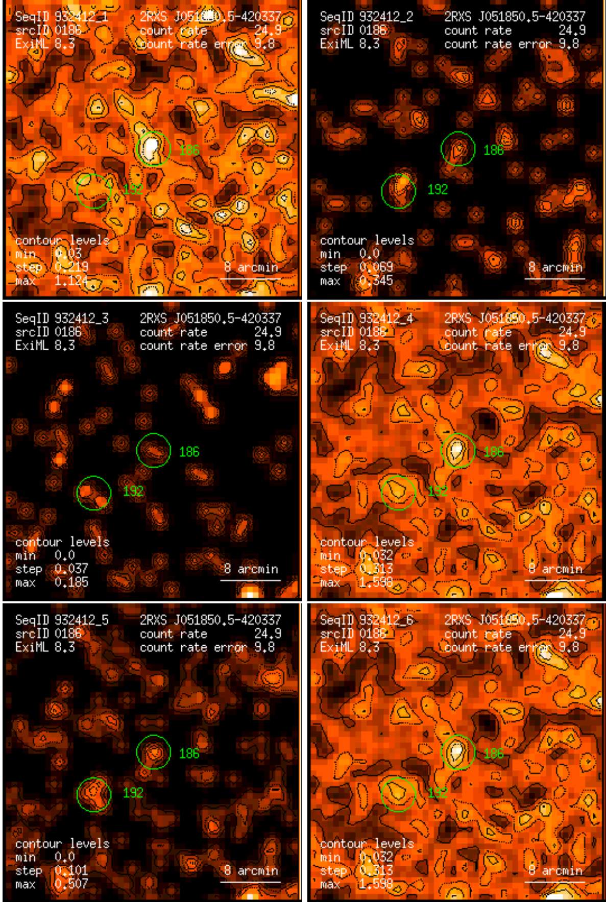
Figure 186: RASS 932412: detection 0186: band rate images, Gaussian filter: (1) PSPC channels 11 – 41, (2) 52 – 90, (3) 91 – 201, (4) 11 – 235, (5) 52 – 201, (6) 11 – 201. Broad band rates in counts/ks. Band rate contour levels in counts/ks/arcmin 2 .
