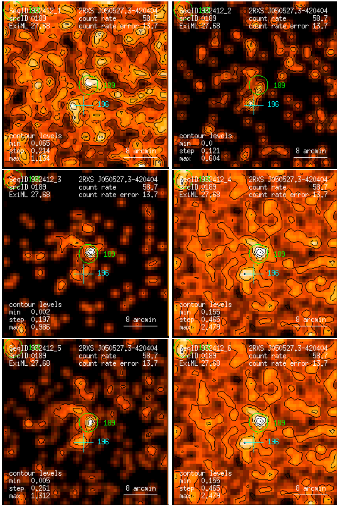
Figure 189: RASS 932412: detection 0189: band rate images, Gaussian filter: (1) PSPC channels 11 – 41, (2) 52 – 90, (3) 91 – 201, (4) 11 – 235, (5) 52 – 201, (6) 11 – 201. Broad band rates in counts/ks. Band rate contour levels in counts/ks/arcmin 2 .
