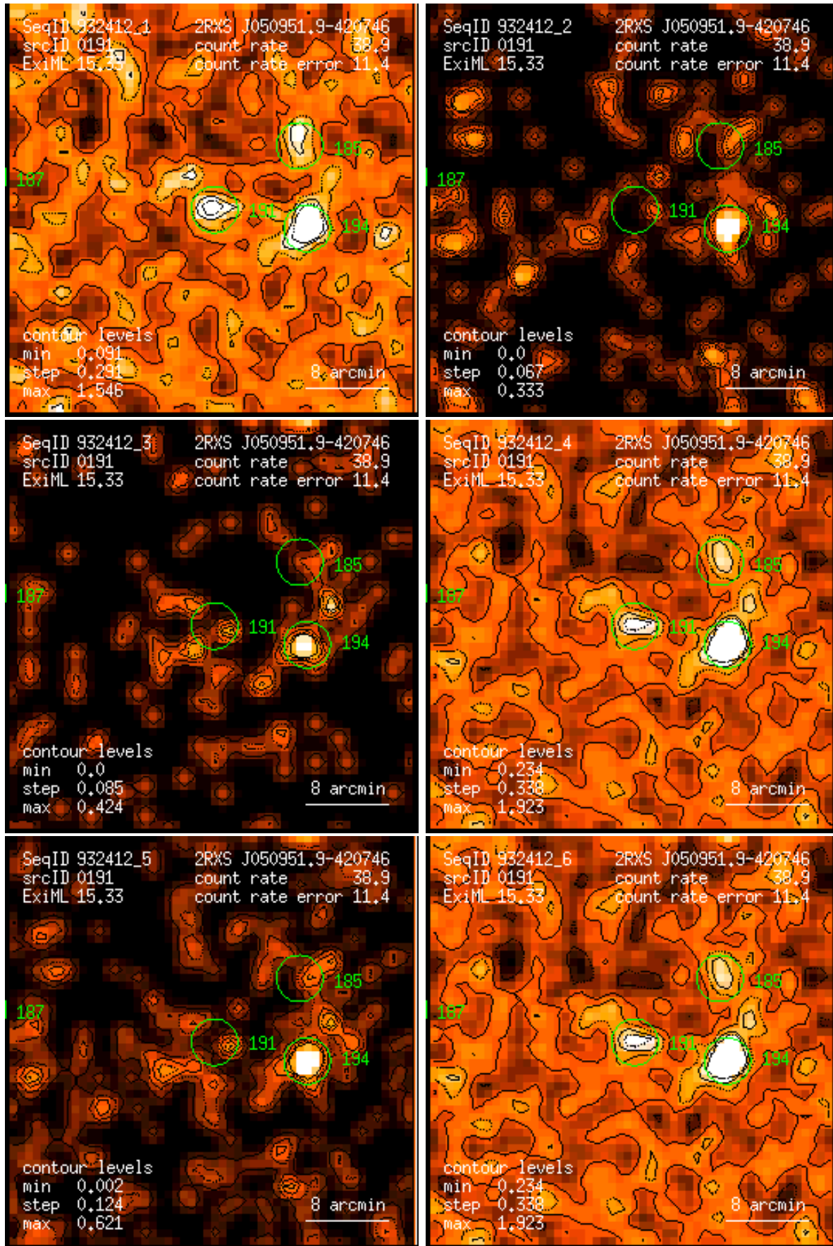
Figure 191: RASS 932412: detection 0191: band rate images, Gaussian filter: (1) PSPC channels 11 – 41, (2) 52 – 90, (3) 91 – 201, (4) 11 – 235, (5) 52 – 201, (6) 11 – 201. Broad band rates in counts/ks. Band rate contour levels in counts/ks/arcmin 2 .
