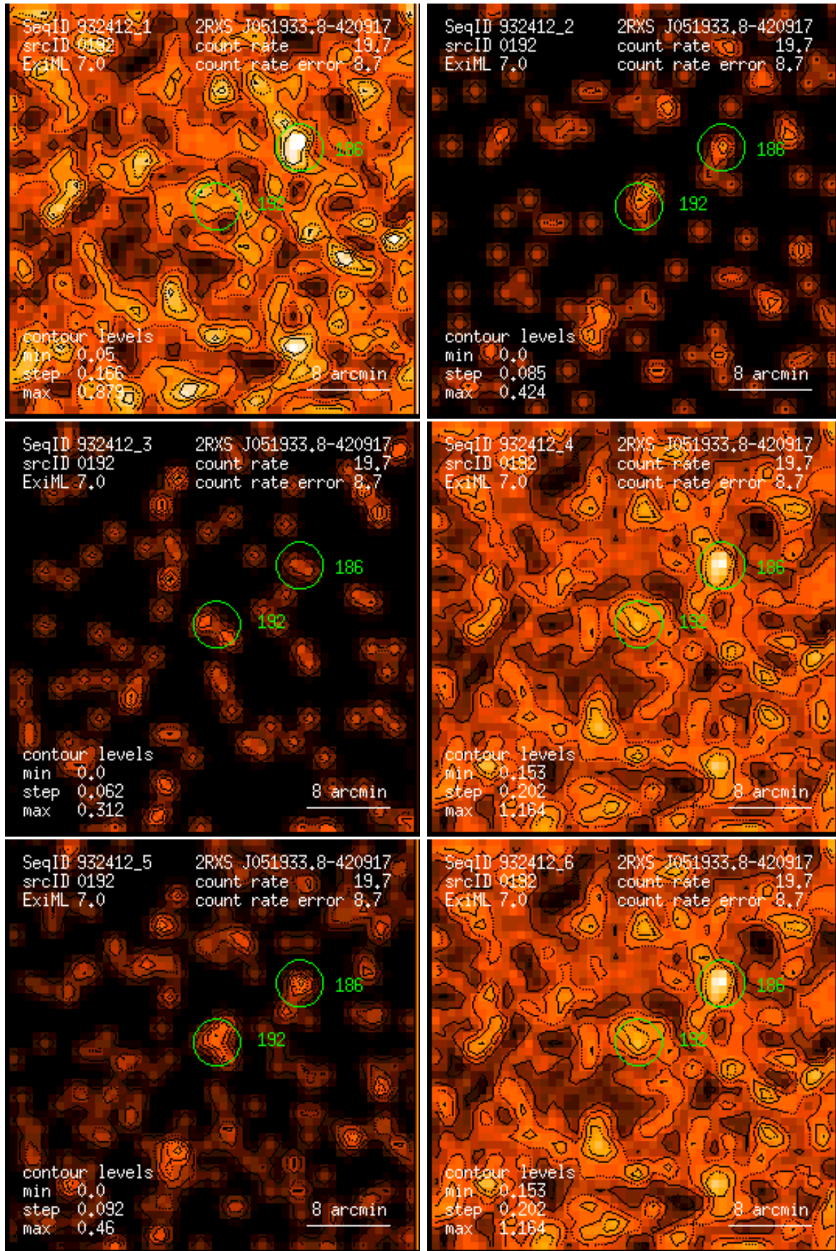
Figure 192: RASS 932412: detection 0192: band rate images, Gaussian filter: (1) PSPC channels 11 – 41, (2) 52 – 90, (3) 91 – 201, (4) 11 – 235, (5) 52 – 201, (6) 11 – 201. Broad band rates in counts/ks. Band rate contour levels in counts/ks/arcmin 2 .
