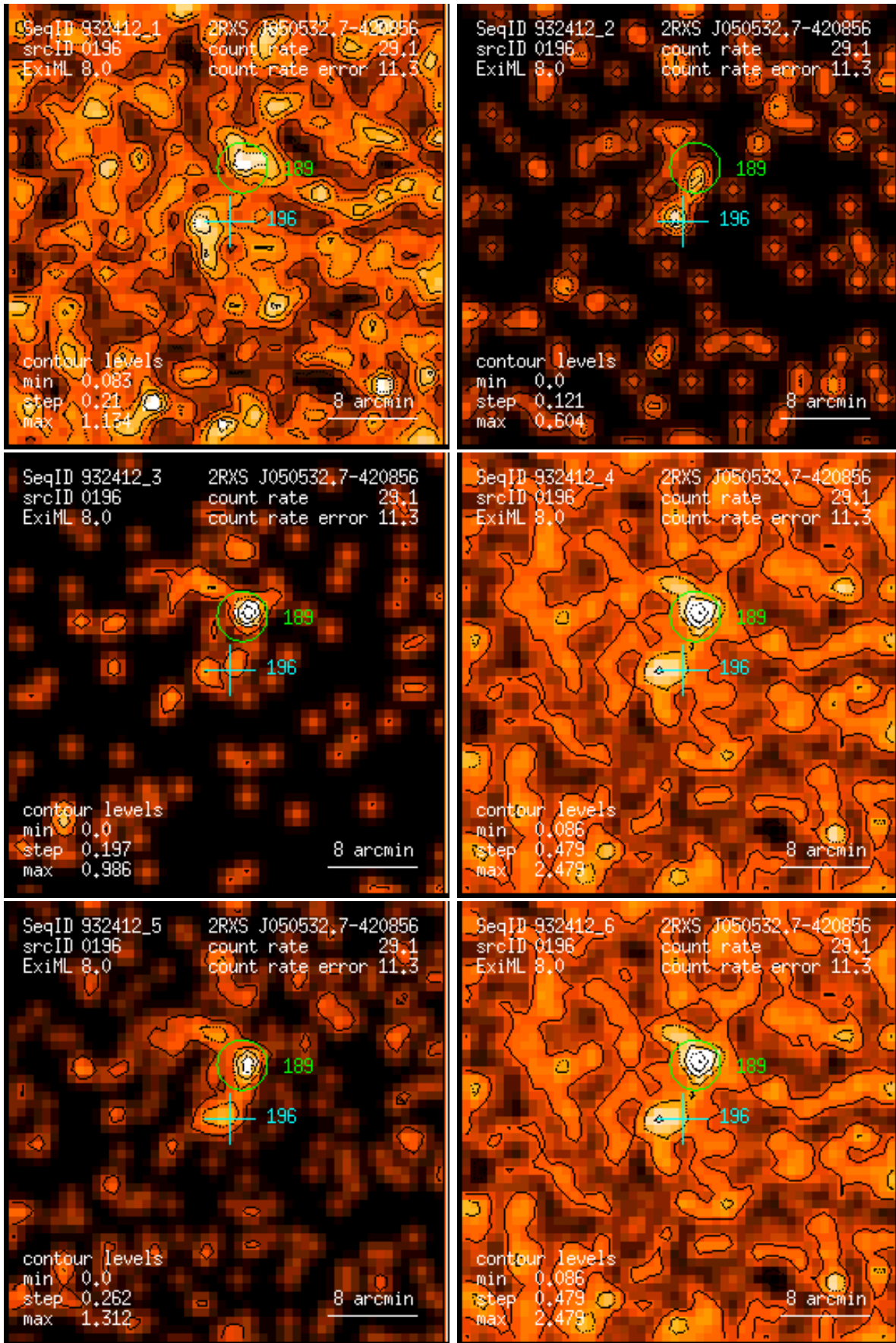
Figure 196: RASS 932412: detection 0196: band rate images, Gaussian filter: (1) PSPC channels 11 – 41, (2) 52 – 90, (3) 91 – 201, (4) 11 – 235, (5) 52 – 201, (6) 11 – 201. Broad band rates in counts/ks. Band rate contour levels in counts/ks/arcmin 2 .
