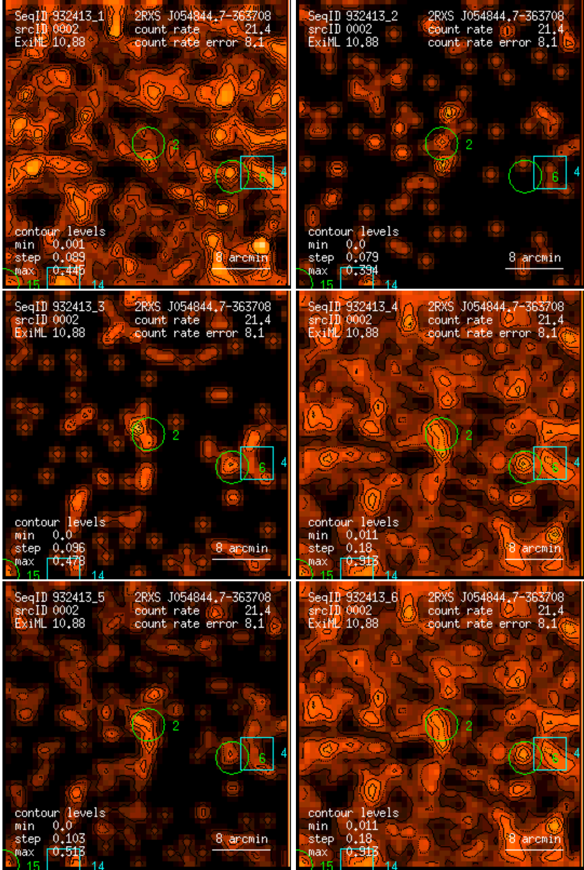
Figure 2: RASS 932413: detection 0002: band rate images, Gaussian filter: (1) PSPC channels 11 – 41, (2) 52 – 90, (3) 91 – 201, (4) 11 – 235, (5) 52 – 201, (6) 11 – 201. Broad band rates in counts/ks. Band rate contour levels in counts/ks/arcmin 2 .
