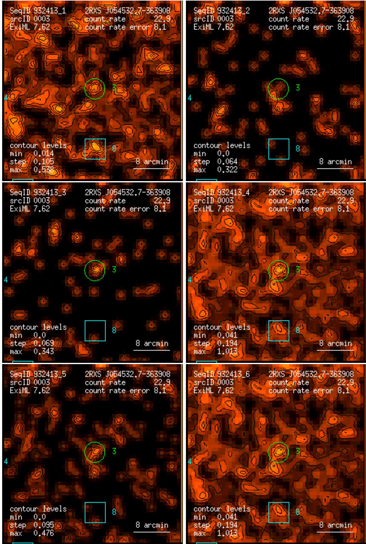
Figure 3: RASS 932413: detection 0003: band rate images, Gaussian filter: (1) PSPC channels 11 – 41, (2) 52 – 90, (3) 91 – 201, (4) 11 – 235, (5) 52 – 201, (6) 11 – 201. Broad band rates in counts/ks. Band rate contour levels in counts/ks/arcmin 2 .
