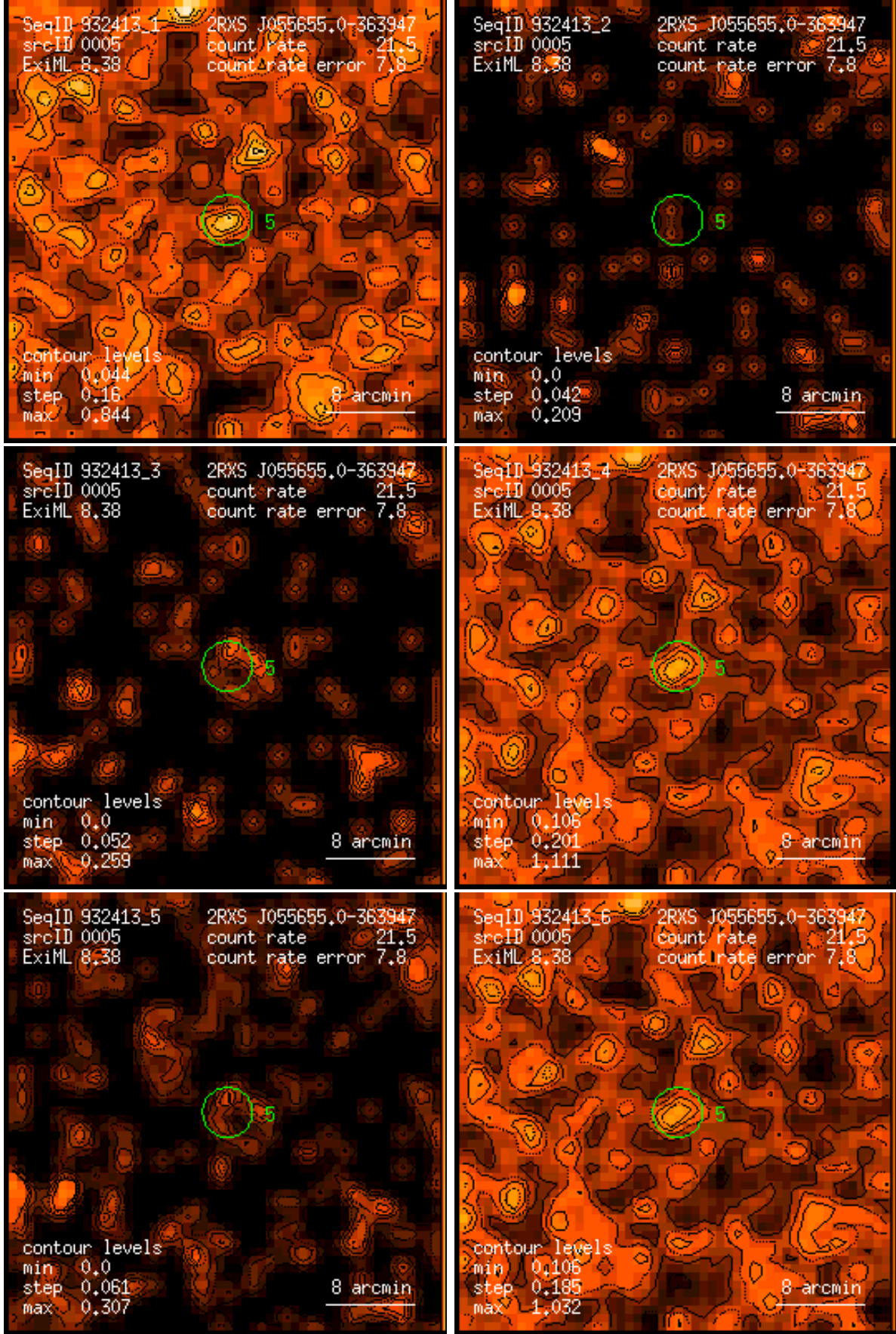
Figure 5: RASS 932413: detection 0005: band rate images, Gaussian filter: (1) PSPC channels 11 – 41, (2) 52 – 90, (3) 91 – 201, (4) 11 – 235, (5) 52 – 201, (6) 11 – 201. Broad band rates in counts/ks. Band rate contour levels in counts/ks/arcmin 2 .
