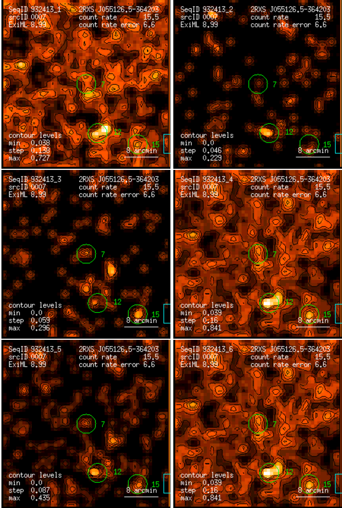
Figure 7: RASS 932413: detection 0007: band rate images, Gaussian filter: (1) PSPC channels 11 – 41, (2) 52 – 90, (3) 91 – 201, (4) 11 – 235, (5) 52 – 201, (6) 11 – 201. Broad band rates in counts/ks. Band rate contour levels in counts/ks/arcmin 2 .
