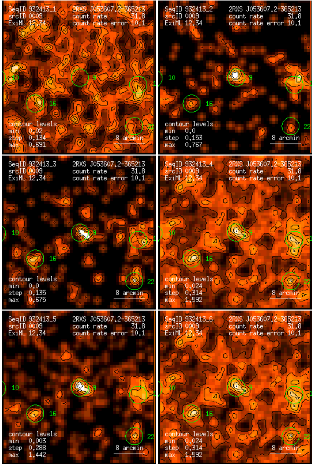
Figure 9: RASS 932413: detection 0009: band rate images, Gaussian filter: (1) PSPC channels 11 – 41, (2) 52 – 90, (3) 91 – 201, (4) 11 – 235, (5) 52 – 201, (6) 11 – 201. Broad band rates in counts/ks. Band rate contour levels in counts/ks/arcmin 2 .
