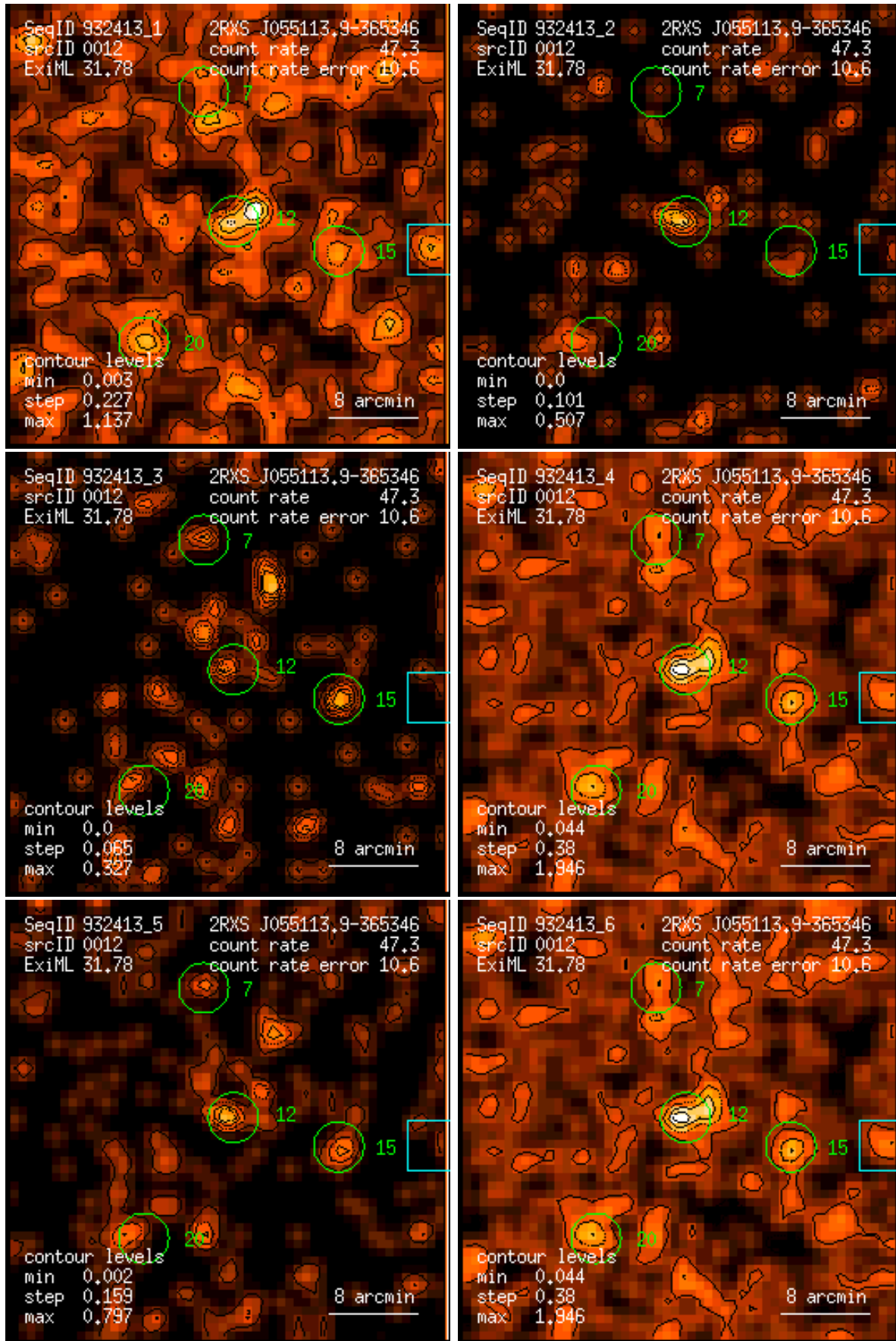
Figure 12: RASS 932413: detection 0012: band rate images, Gaussian filter: (1) PSPC channels 11 – 41, (2) 52 – 90, (3) 91 – 201, (4) 11 – 235, (5) 52 – 201, (6) 11 – 201. Broad band rates in counts/ks. Band rate contour levels in counts/ks/arcmin 2 .
