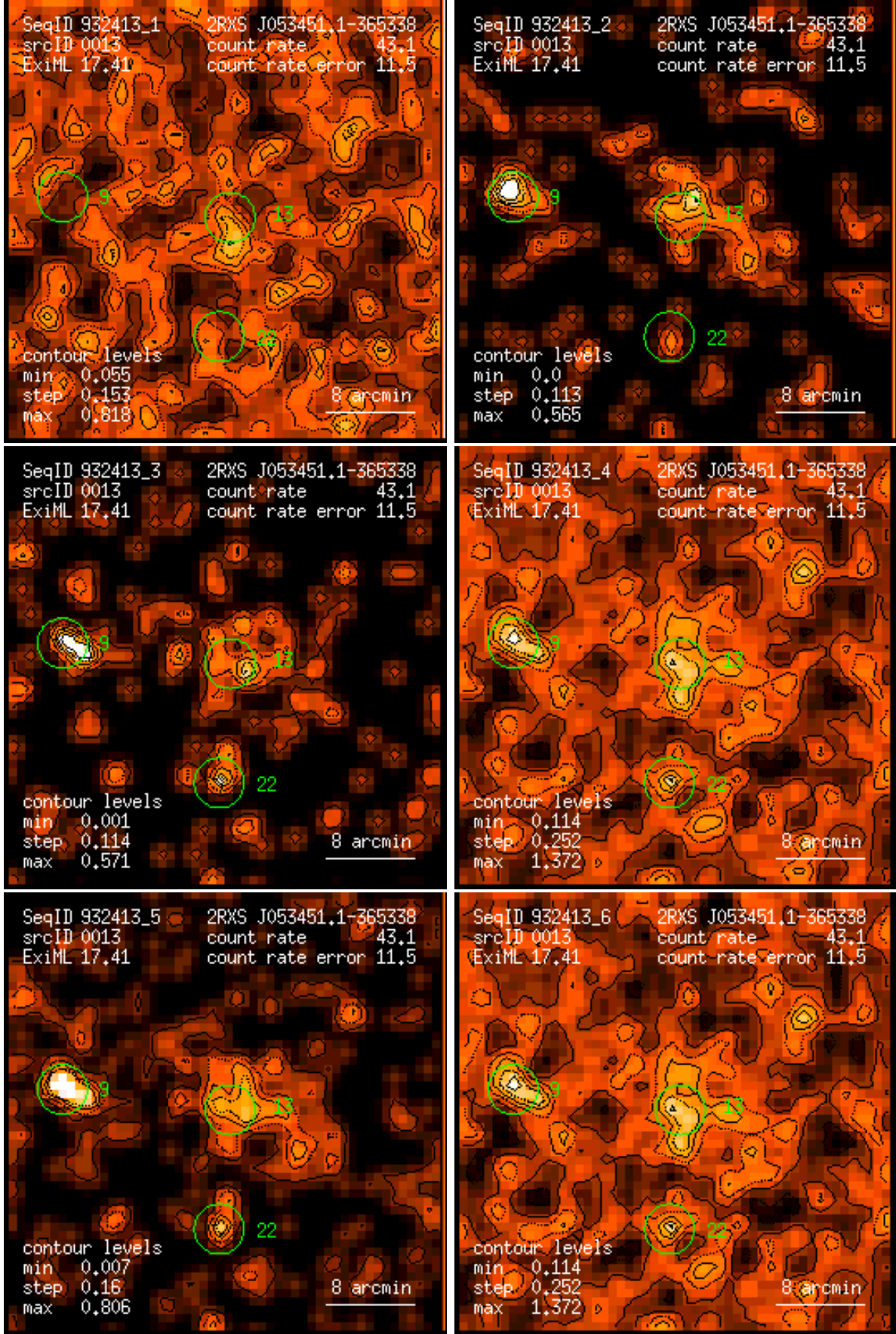
Figure 13: RASS 932413: detection 0013: band rate images, Gaussian filter: (1) PSPC channels 11 – 41, (2) 52 – 90, (3) 91 – 201, (4) 11 – 235, (5) 52 – 201, (6) 11 – 201. Broad band rates in counts/ks. Band rate contour levels in counts/ks/arcmin 2 .
