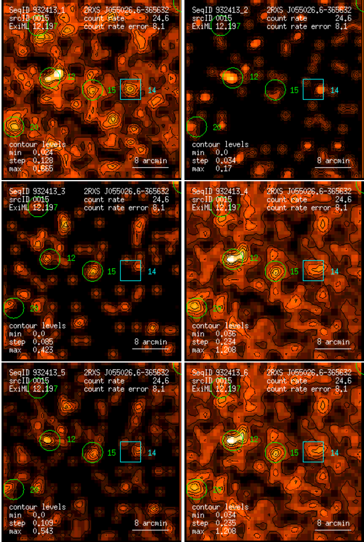
Figure 15: RASS 932413: detection 0015: band rate images, Gaussian filter: (1) PSPC channels 11 – 41, (2) 52 – 90, (3) 91 – 201, (4) 11 – 235, (5) 52 – 201, (6) 11 – 201. Broad band rates in counts/ks. Band rate contour levels in counts/ks/arcmin 2 .
