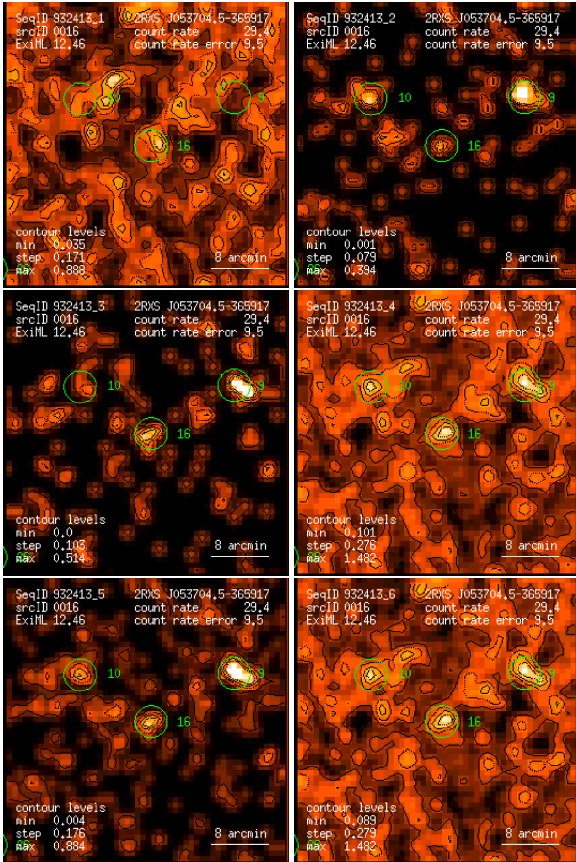
Figure 16: RASS 932413: detection 0016: band rate images, Gaussian filter: (1) PSPC channels 11 – 41, (2) 52 – 90, (3) 91 – 201, (4) 11 – 235, (5) 52 – 201, (6) 11 – 201. Broad band rates in counts/ks. Band rate contour levels in counts/ks/arcmin 2 .
