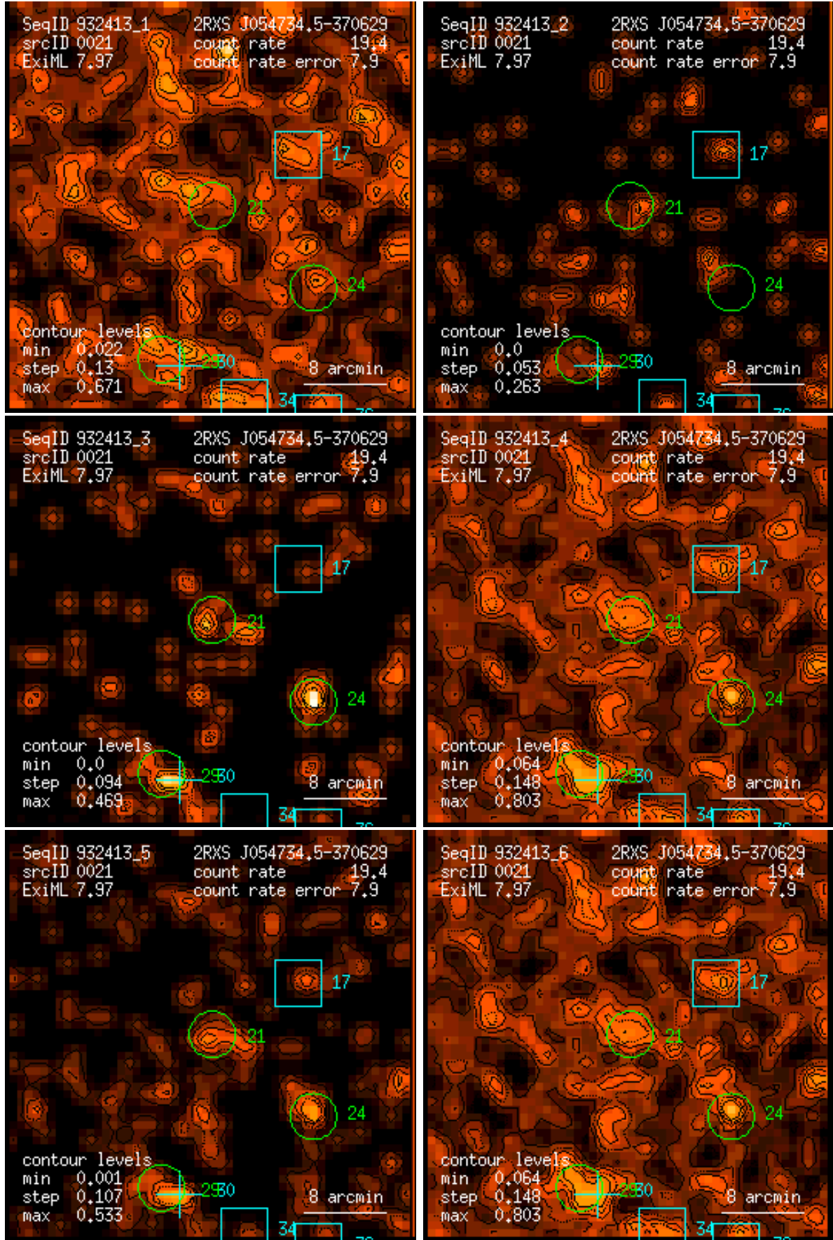
Figure 21: RASS 932413: detection 0021: band rate images, Gaussian filter: (1) PSPC channels 11 – 41, (2) 52 – 90, (3) 91 – 201, (4) 11 – 235, (5) 52 – 201, (6) 11 – 201. Broad band rates in counts/ks. Band rate contour levels in counts/ks/arcmin 2 .
