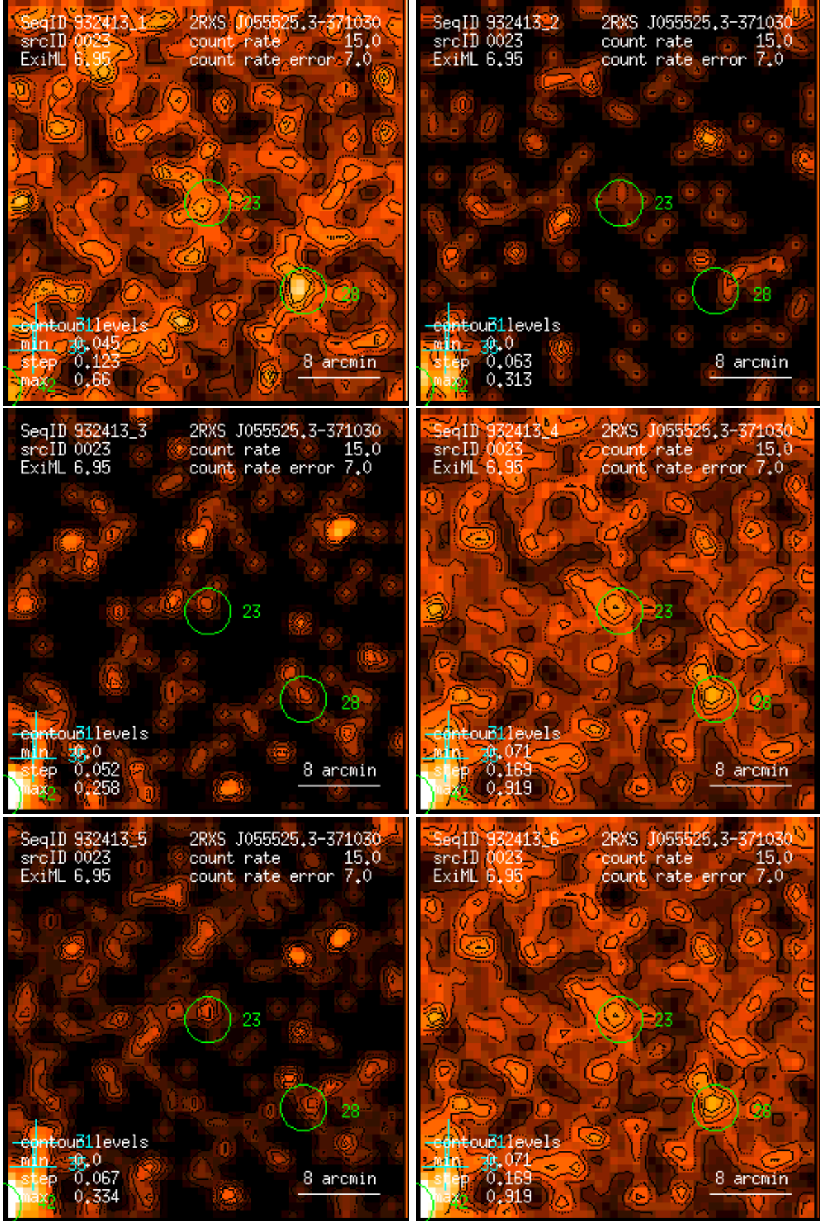
Figure 23: RASS 932413: detection 0023: band rate images, Gaussian filter: (1) PSPC channels 11 – 41, (2) 52 – 90, (3) 91 – 201, (4) 11 – 235, (5) 52 – 201, (6) 11 – 201. Broad band rates in counts/ks. Band rate contour levels in counts/ks/arcmin 2 .
