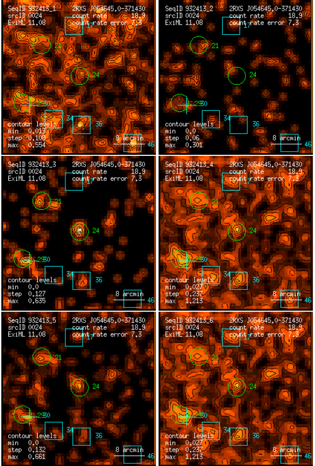
Figure 24: RASS 932413: detection 0024: band rate images, Gaussian filter: (1) PSPC channels 11 – 41, (2) 52 – 90, (3) 91 – 201, (4) 11 – 235, (5) 52 – 201, (6) 11 – 201. Broad band rates in counts/ks. Band rate contour levels in counts/ks/arcmin 2 .
