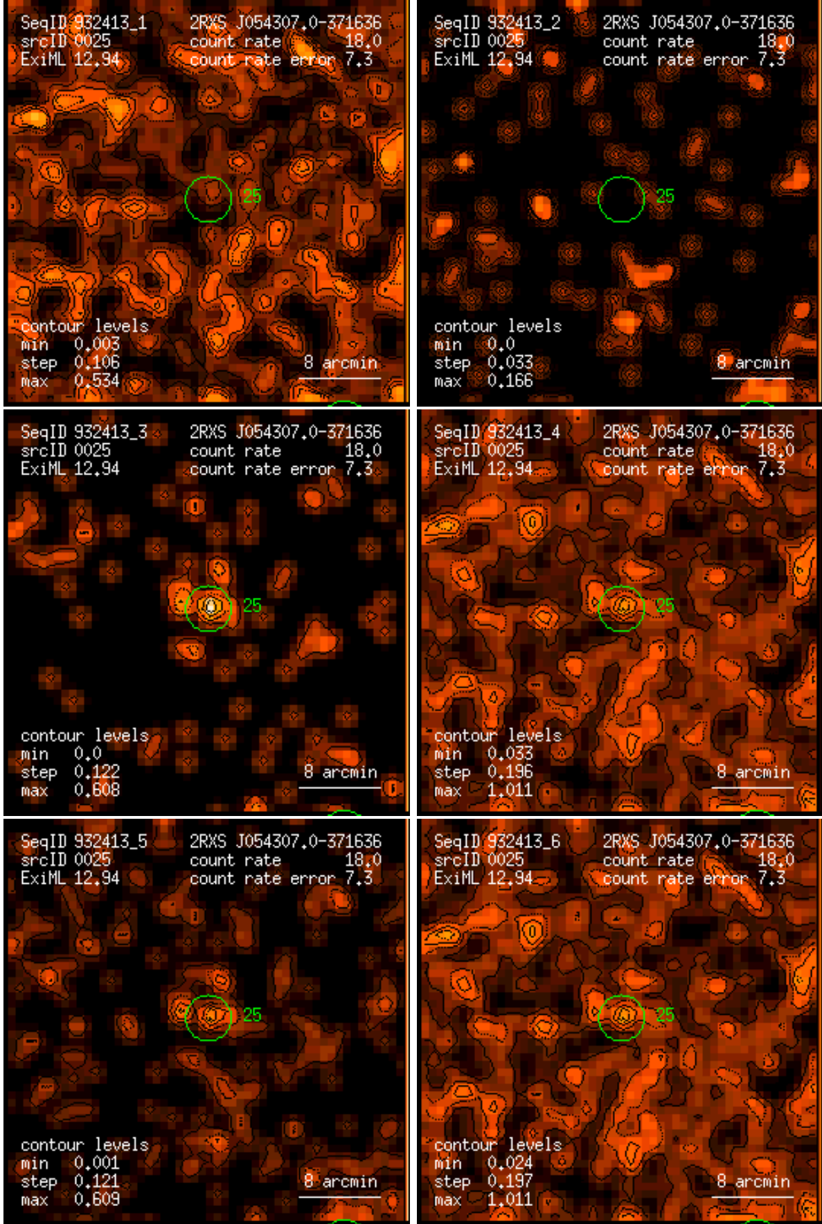
Figure 25: RASS 932413: detection 0025: band rate images, Gaussian filter: (1) PSPC channels 11 – 41, (2) 52 – 90, (3) 91 – 201, (4) 11 – 235, (5) 52 – 201, (6) 11 – 201. Broad band rates in counts/ks. Band rate contour levels in counts/ks/arcmin 2 .
