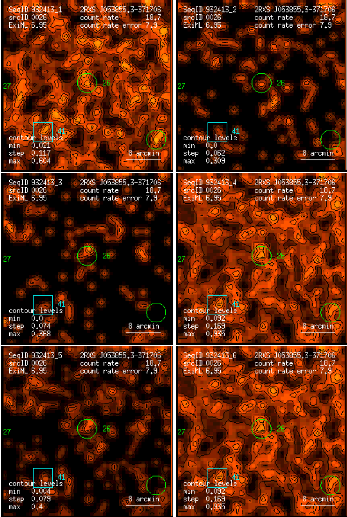
Figure 26: RASS 932413: detection 0026: band rate images, Gaussian filter: (1) PSPC channels 11 – 41, (2) 52 – 90, (3) 91 – 201, (4) 11 – 235, (5) 52 – 201, (6) 11 – 201. Broad band rates in counts/ks. Band rate contour levels in counts/ks/arcmin 2 .
