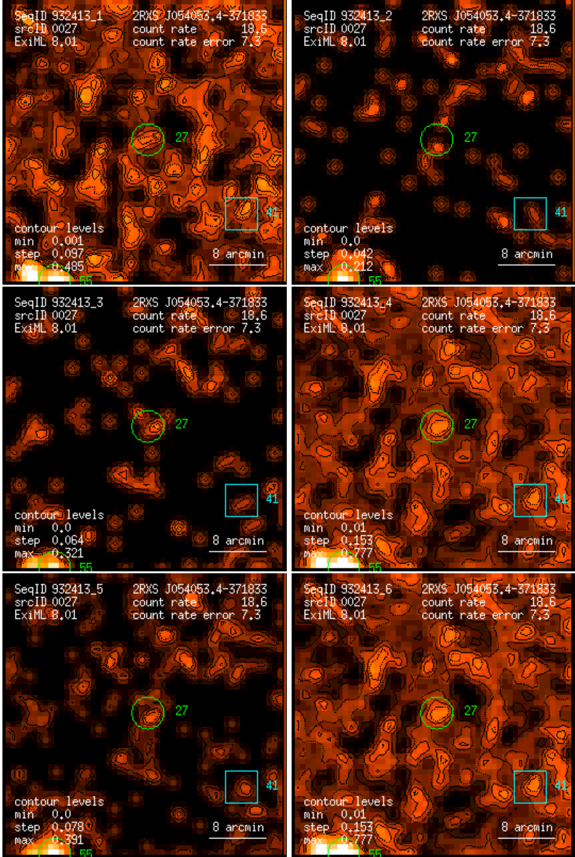
Figure 27: RASS 932413: detection 0027: band rate images, Gaussian filter: (1) PSPC channels 11 – 41, (2) 52 – 90, (3) 91 – 201, (4) 11 – 235, (5) 52 – 201, (6) 11 – 201. Broad band rates in counts/ks. Band rate contour levels in counts/ks/arcmin 2 .
