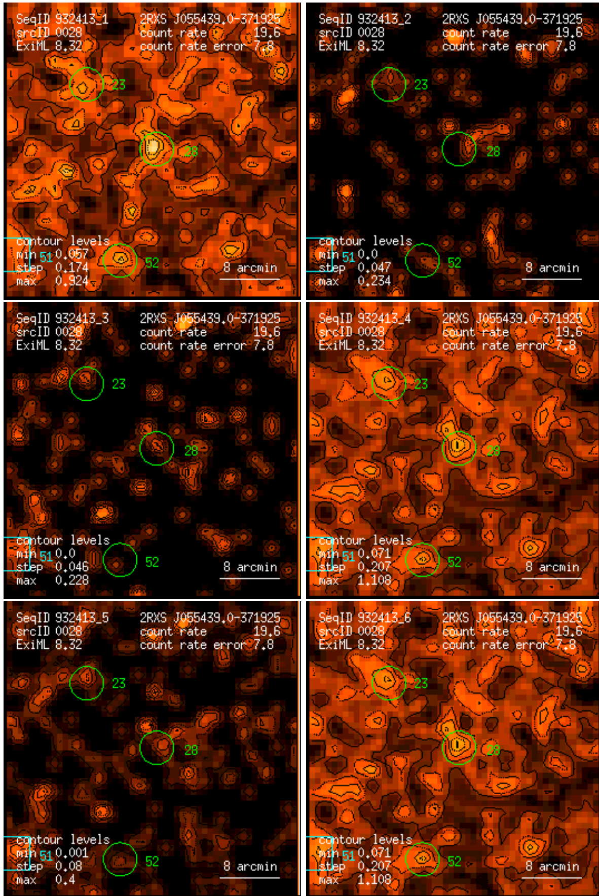
Figure 28: RASS 932413: detection 0028: band rate images, Gaussian filter: (1) PSPC channels 11 – 41, (2) 52 – 90, (3) 91 – 201, (4) 11 – 235, (5) 52 – 201, (6) 11 – 201. Broad band rates in counts/ks. Band rate contour levels in counts/ks/arcmin 2 .
