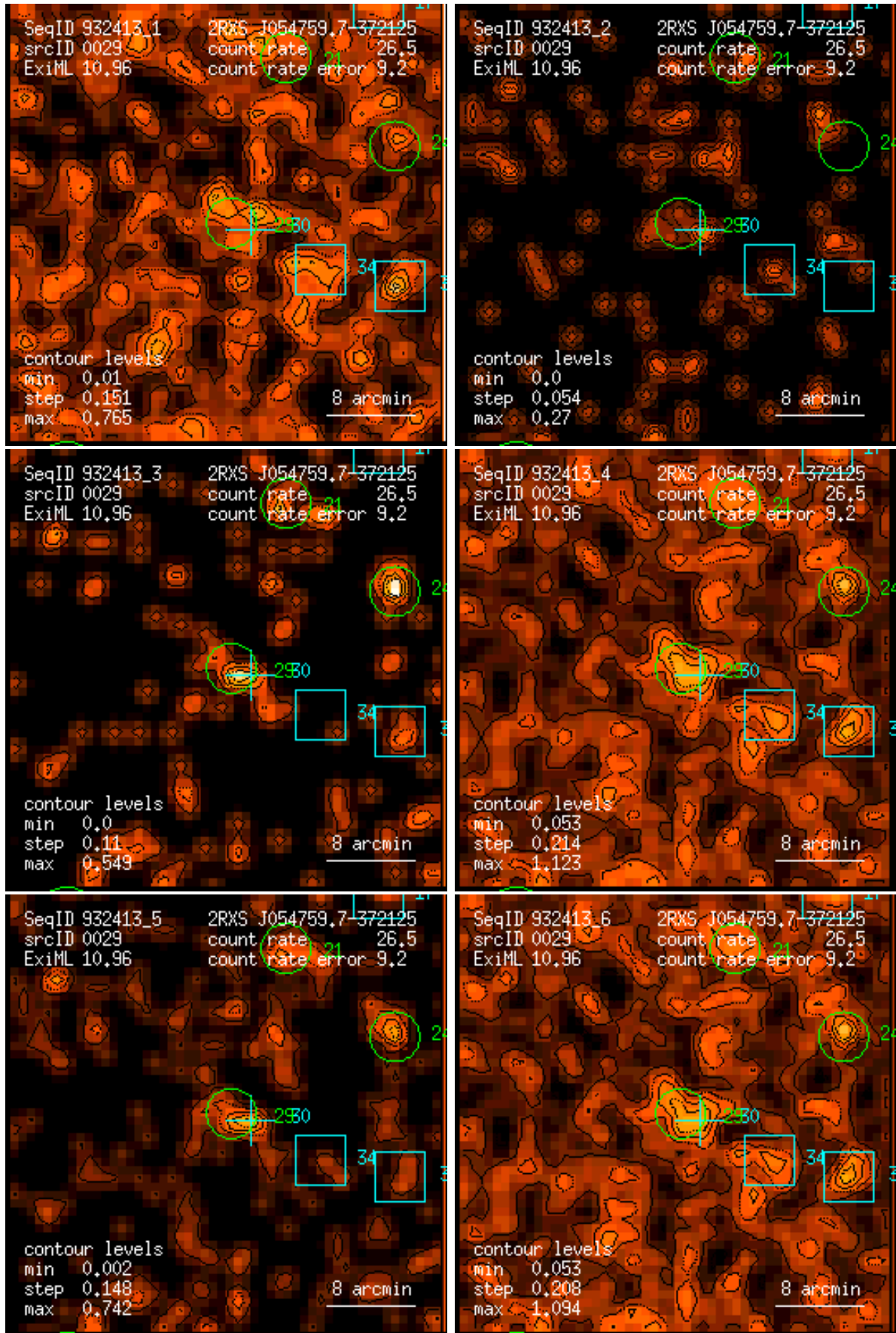
Figure 29: RASS 932413: detection 0029: band rate images, Gaussian filter: (1) PSPC channels 11 – 41, (2) 52 – 90, (3) 91 – 201, (4) 11 – 235, (5) 52 – 201, (6) 11 – 201. Broad band rates in counts/ks. Band rate contour levels in counts/ks/arcmin 2 .
