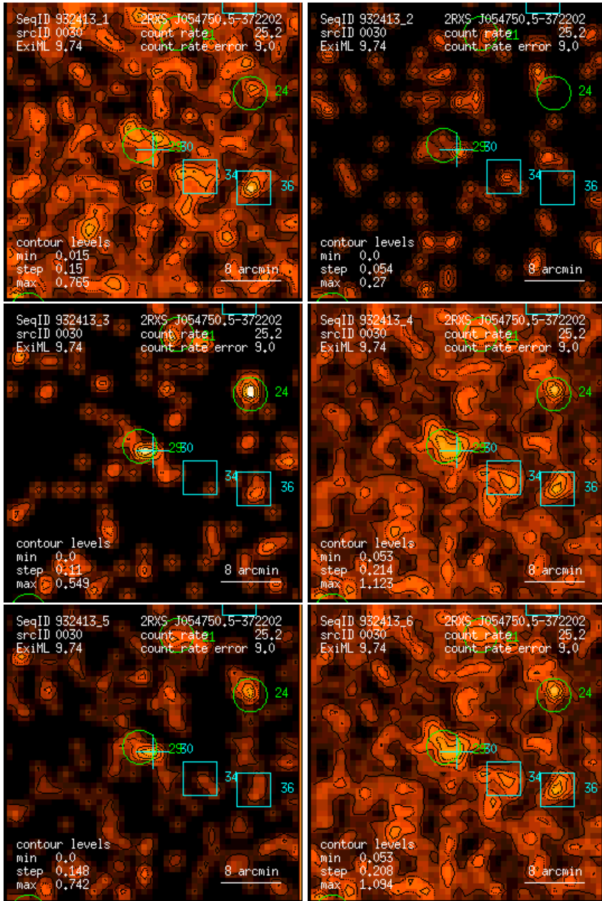
Figure 30: RASS 932413: detection 0030: band rate images, Gaussian filter: (1) PSPC channels 11 – 41, (2) 52 – 90, (3) 91 – 201, (4) 11 – 235, (5) 52 – 201, (6) 11 – 201. Broad band rates in counts/ks. Band rate contour levels in counts/ks/arcmin 2 .
