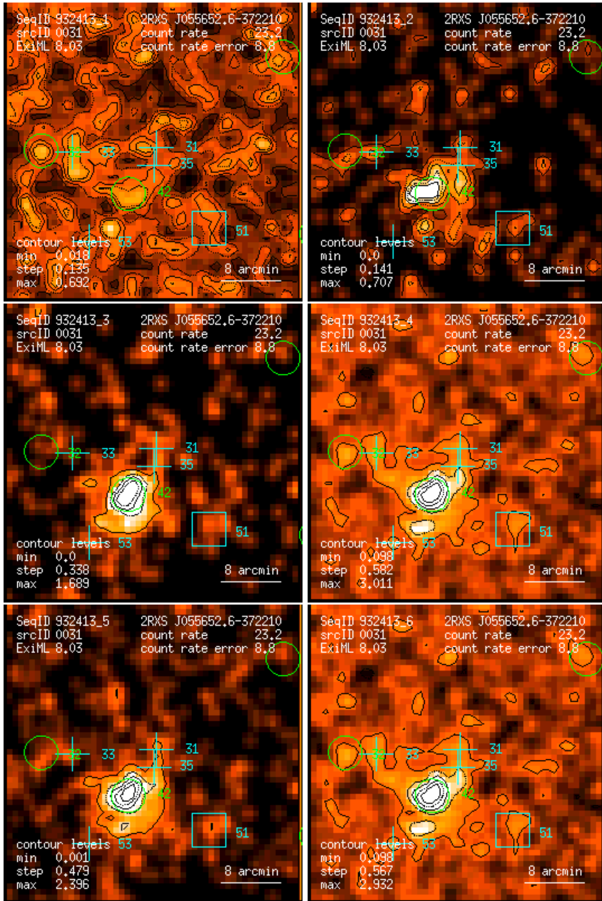
Figure 31: RASS 932413: detection 0031: band rate images, Gaussian filter: (1) PSPC channels 11 – 41, (2) 52 – 90, (3) 91 – 201, (4) 11 – 235, (5) 52 – 201, (6) 11 – 201. Broad band rates in counts/ks. Band rate contour levels in counts/ks/arcmin 2 .
