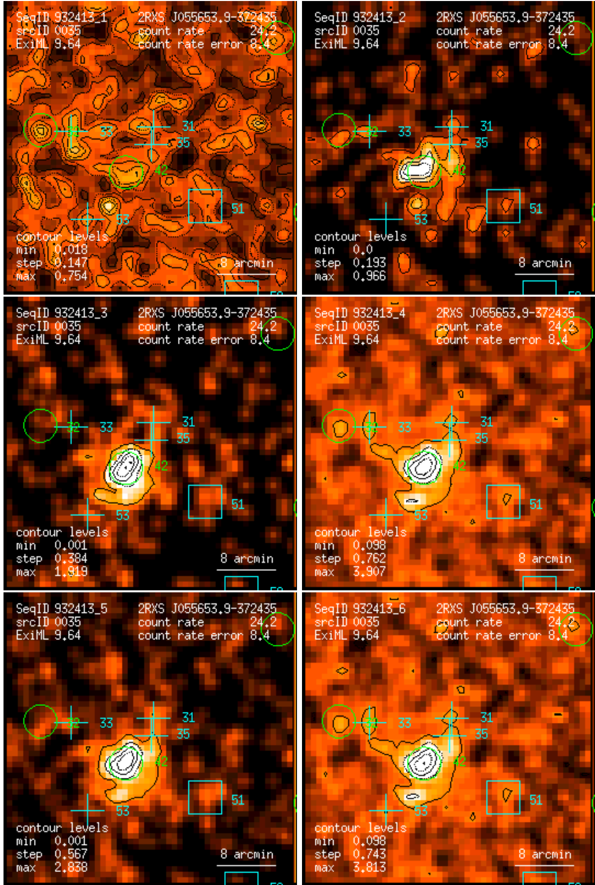
Figure 35: RASS 932413: detection 0035: band rate images, Gaussian filter: (1) PSPC channels 11 – 41, (2) 52 – 90, (3) 91 – 201, (4) 11 – 235, (5) 52 – 201, (6) 11 – 201. Broad band rates in counts/ks. Band rate contour levels in counts/ks/arcmin 2 .
