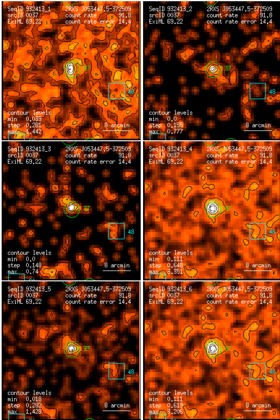
Figure 37: RASS 932413: detection 0037: band rate images, Gaussian filter: (1) PSPC channels 11 – 41, (2) 52 – 90, (3) 91 – 201, (4) 11 – 235, (5) 52 – 201, (6) 11 – 201. Broad band rates in counts/ks. Band rate contour levels in counts/ks/arcmin 2 .
