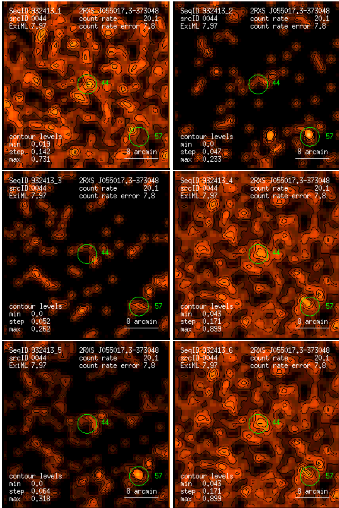
Figure 44: RASS 932413: detection 0044: band rate images, Gaussian filter: (1) PSPC channels 11 – 41, (2) 52 – 90, (3) 91 – 201, (4) 11 – 235, (5) 52 – 201, (6) 11 – 201. Broad band rates in counts/ks. Band rate contour levels in counts/ks/arcmin 2 .
