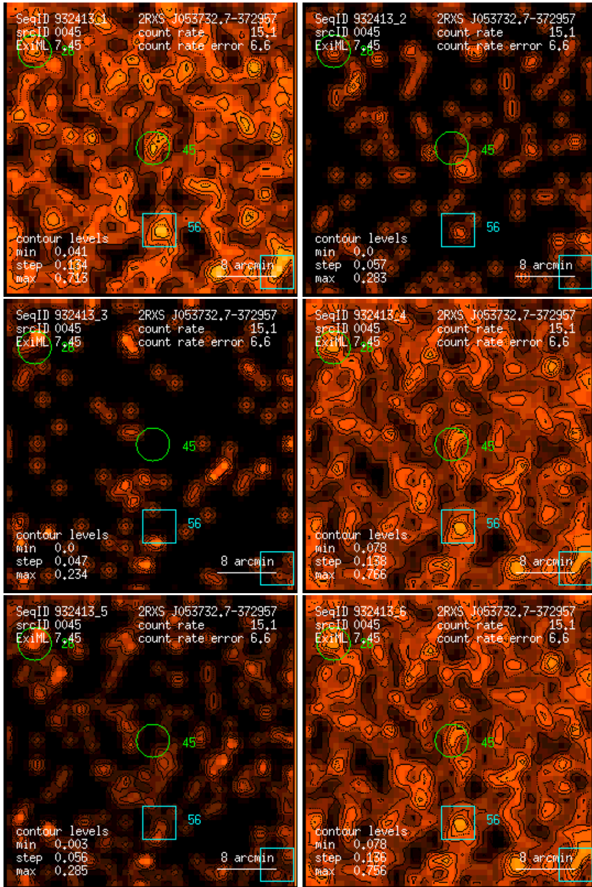
Figure 45: RASS 932413: detection 0045: band rate images, Gaussian filter: (1) PSPC channels 11 – 41, (2) 52 – 90, (3) 91 – 201, (4) 11 – 235, (5) 52 – 201, (6) 11 – 201. Broad band rates in counts/ks. Band rate contour levels in counts/ks/arcmin 2 .
