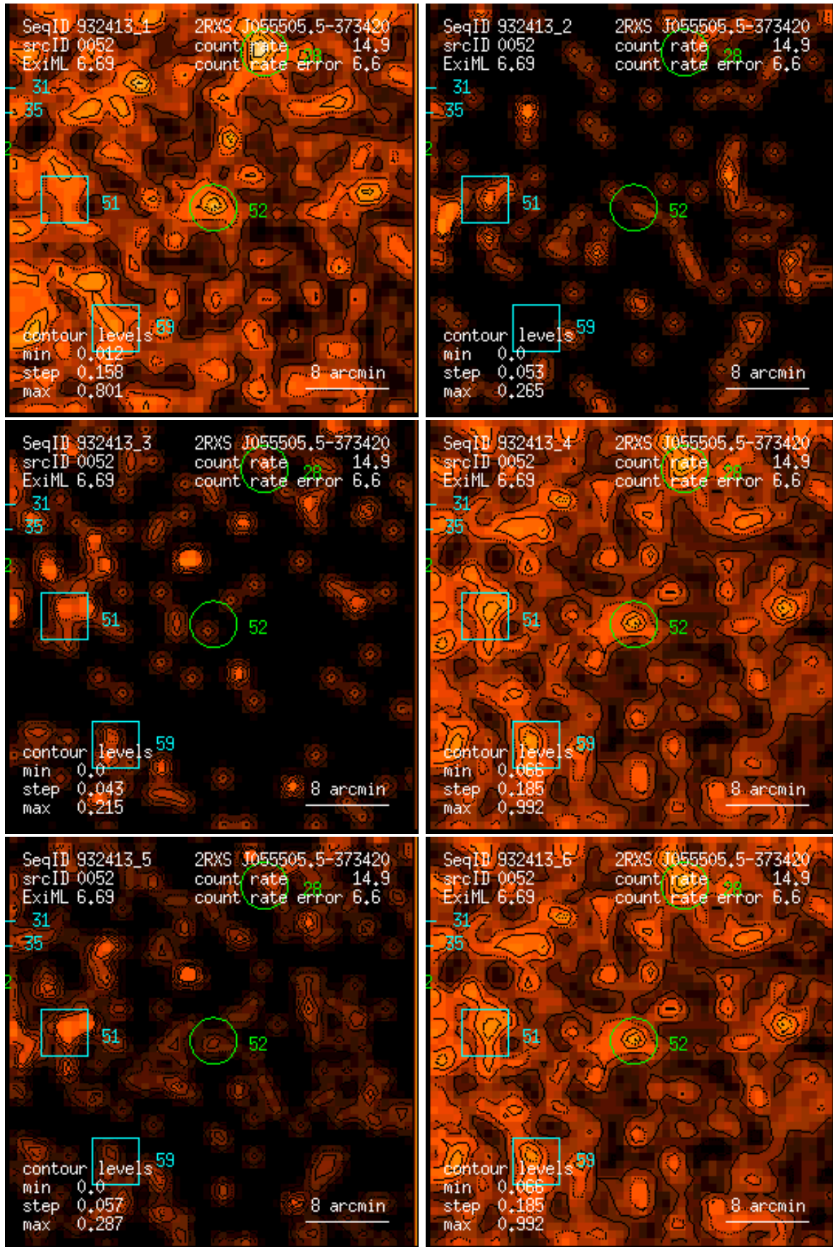
Figure 52: RASS 932413: detection 0052: band rate images, Gaussian filter: (1) PSPC channels 11 – 41, (2) 52 – 90, (3) 91 – 201, (4) 11 – 235, (5) 52 – 201, (6) 11 – 201. Broad band rates in counts/ks. Band rate contour levels in counts/ks/arcmin 2 .
