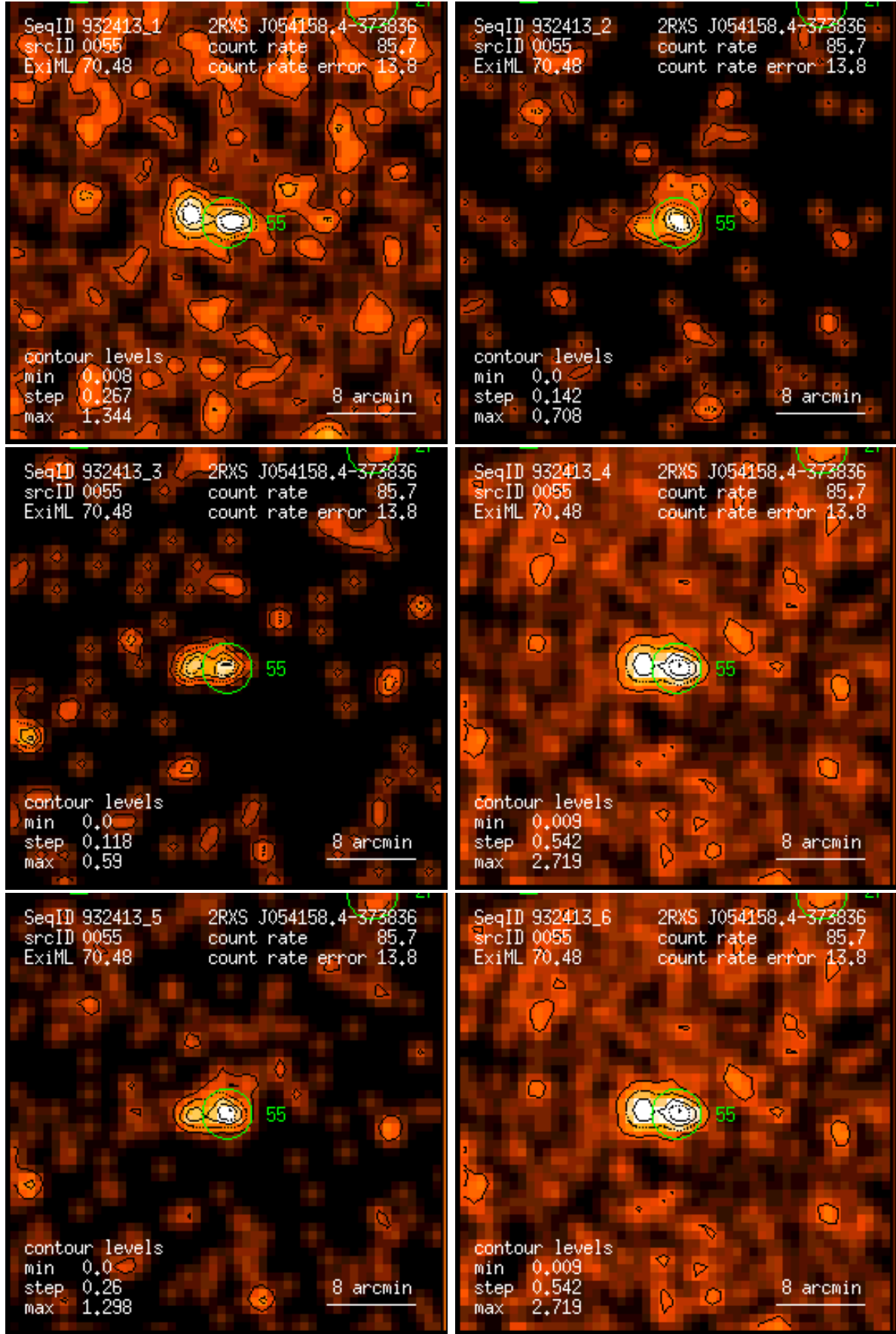
Figure 55: RASS 932413: detection 0055: band rate images, Gaussian filter: (1) PSPC channels 11 – 41, (2) 52 – 90, (3) 91 – 201, (4) 11 – 235, (5) 52 – 201, (6) 11 – 201. Broad band rates in counts/ks. Band rate contour levels in counts/ks/arcmin 2 .
