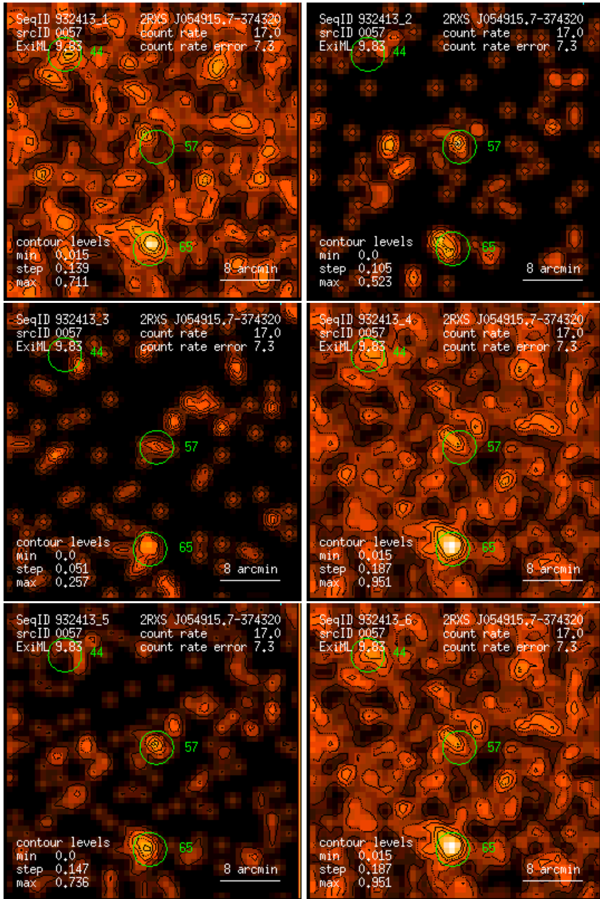
Figure 57: RASS 932413: detection 0057: band rate images, Gaussian filter: (1) PSPC channels 11 – 41, (2) 52 – 90, (3) 91 – 201, (4) 11 – 235, (5) 52 – 201, (6) 11 – 201. Broad band rates in counts/ks. Band rate contour levels in counts/ks/arcmin 2 .
