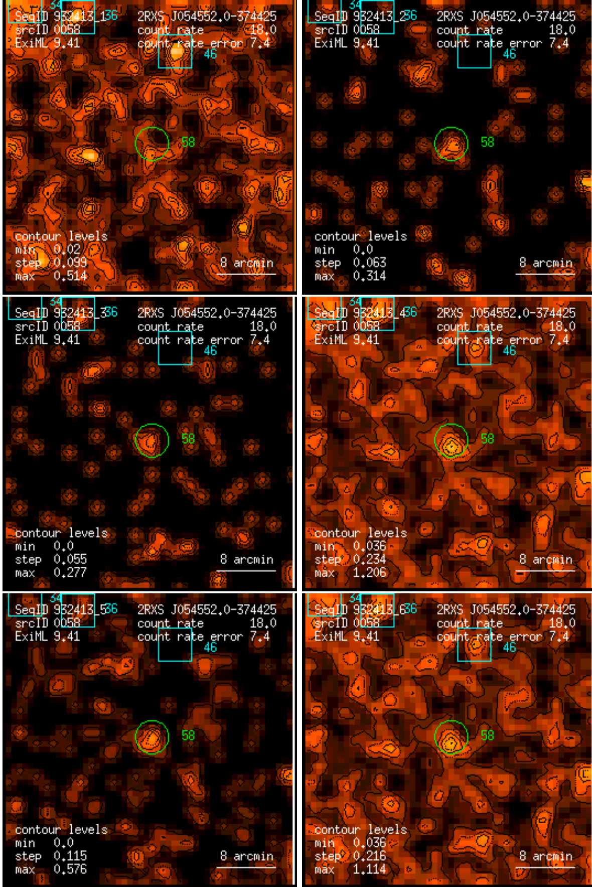
Figure 58: RASS 932413: detection 0058: band rate images, Gaussian filter: (1) PSPC channels 11 – 41, (2) 52 – 90, (3) 91 – 201, (4) 11 – 235, (5) 52 – 201, (6) 11 – 201. Broad band rates in counts/ks. Band rate contour levels in counts/ks/arcmin 2 .
