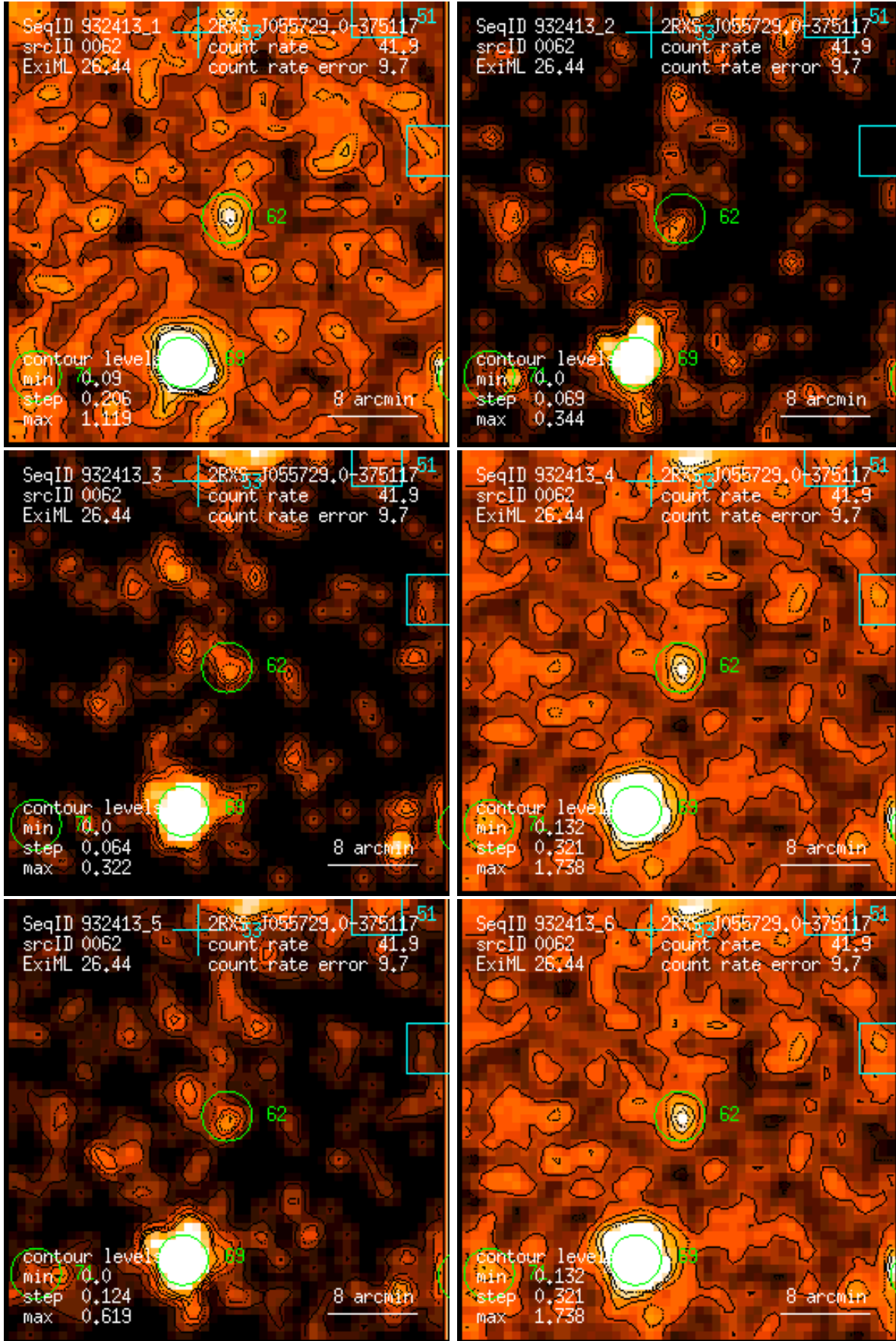
Figure 62: RASS 932413: detection 0062: band rate images, Gaussian filter: (1) PSPC channels 11 – 41, (2) 52 – 90, (3) 91 – 201, (4) 11 – 235, (5) 52 – 201, (6) 11 – 201. Broad band rates in counts/ks. Band rate contour levels in counts/ks/arcmin 2 .
