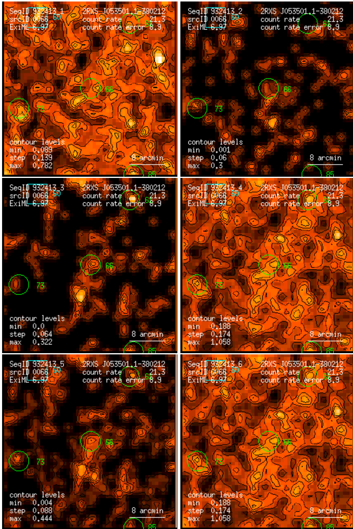
Figure 66: RASS 932413: detection 0066: band rate images, Gaussian filter: (1) PSPC channels 11 – 41, (2) 52 – 90, (3) 91 – 201, (4) 11 – 235, (5) 52 – 201, (6) 11 – 201. Broad band rates in counts/ks. Band rate contour levels in counts/ks/arcmin 2 .
