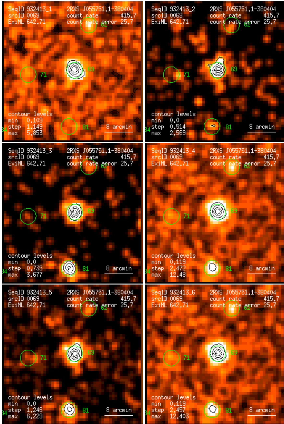
Figure 69: RASS 932413: detection 0069: band rate images, Gaussian filter: (1) PSPC channels 11 – 41, (2) 52 – 90, (3) 91 – 201, (4) 11 – 235, (5) 52 – 201, (6) 11 – 201. Broad band rates in counts/ks. Band rate contour levels in counts/ks/arcmin 2 .
