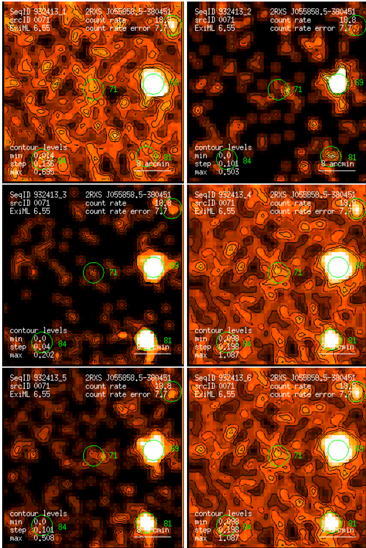
Figure 71: RASS 932413: detection 0071: band rate images, Gaussian filter: (1) PSPC channels 11 – 41, (2) 52 – 90, (3) 91 – 201, (4) 11 – 235, (5) 52 – 201, (6) 11 – 201. Broad band rates in counts/ks. Band rate contour levels in counts/ks/arcmin 2 .
