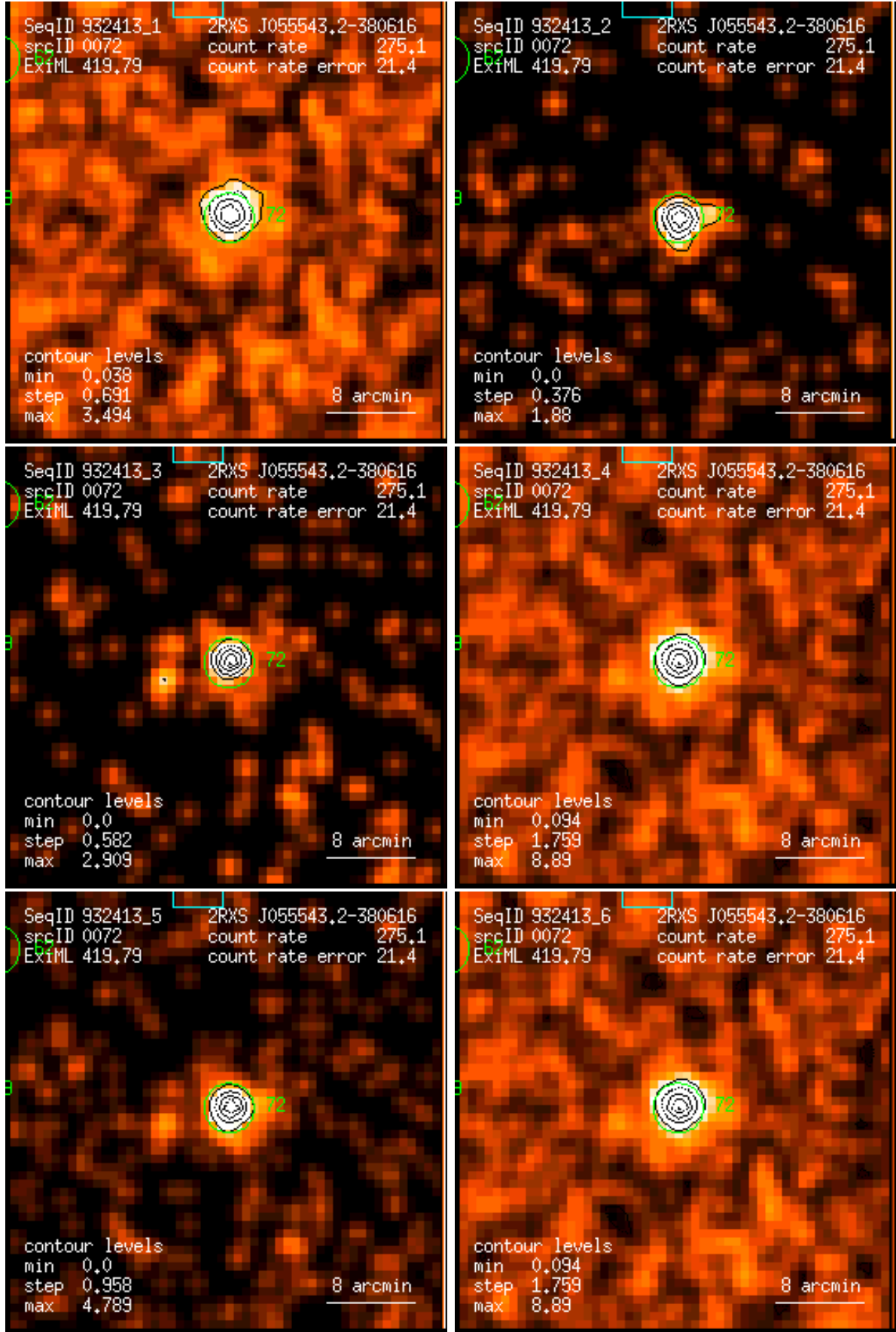
Figure 72: RASS 932413: detection 0072: band rate images, Gaussian filter: (1) PSPC channels 11 – 41, (2) 52 – 90, (3) 91 – 201, (4) 11 – 235, (5) 52 – 201, (6) 11 – 201. Broad band rates in counts/ks. Band rate contour levels in counts/ks/arcmin 2 .
