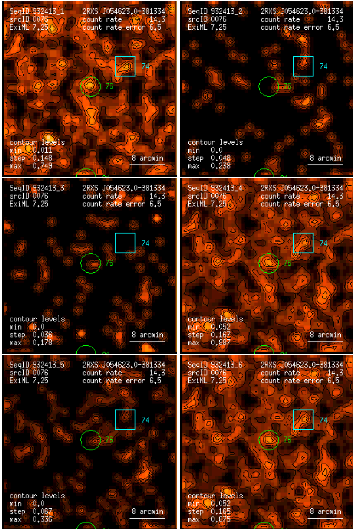
Figure 76: RASS 932413: detection 0076: band rate images, Gaussian filter: (1) PSPC channels 11 – 41, (2) 52 – 90, (3) 91 – 201, (4) 11 – 235, (5) 52 – 201, (6) 11 – 201. Broad band rates in counts/ks. Band rate contour levels in counts/ks/arcmin 2 .
